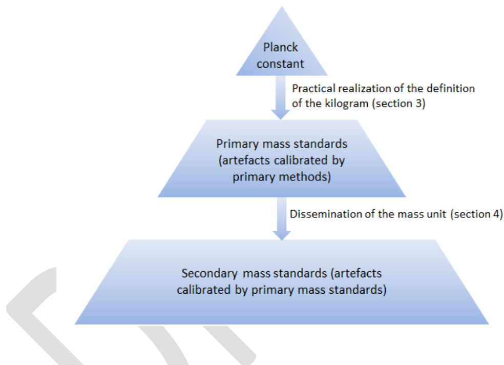
Figure 1. Illustration of the traceability chain from the definition of the kilogram. The unit of the Planck constant being \text{kg m}^2 \text{s}^{-1} , the units second and metre are needed to derive a primary mass standard from the Planck constant.
