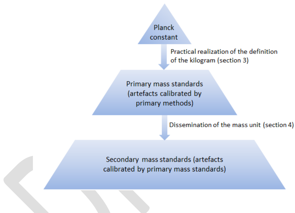
Figure 1. Illustration of the traceability chain from the definition of the kilogram. The unit of the Planck constant being \text{kg m}^2 \text{s}^{-1} , the units second and metre are needed to derive a primary mass standard from the Planck constant.
