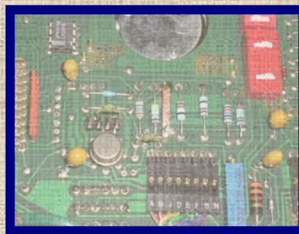
Modification of the electrometer circuit board
