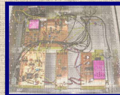
Complete measurement chain
