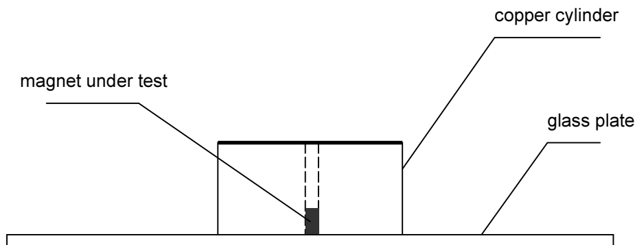
Figure 2. Schematic of sample holder.
