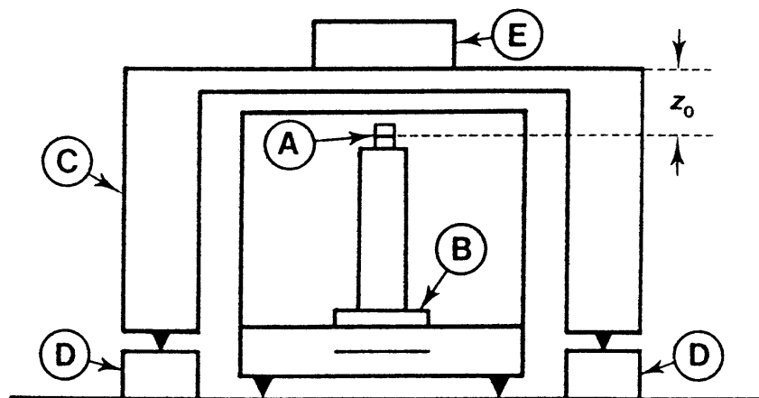
Figure 3. The BIPM susceptometer configured for measuring magnetic susceptibility. A: magnet A; B: balance pan; C: sample support; D: blocks to adjust the height of E with respect to A; E: the sample under test.
