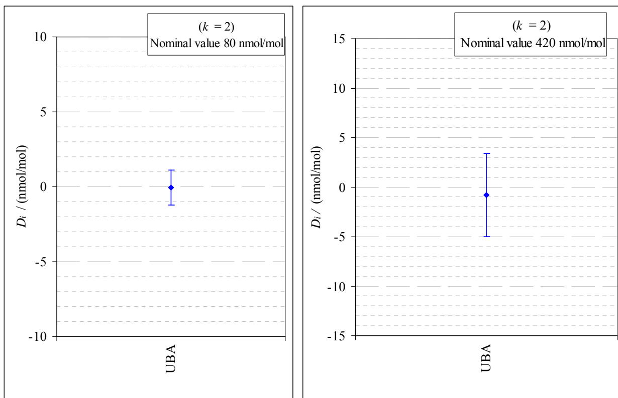
Figure 1: degrees of equivalence of the UBA at the two nominal ozone amount-of-substance fractions 80 nmol/mol and 420 nmol/mol
