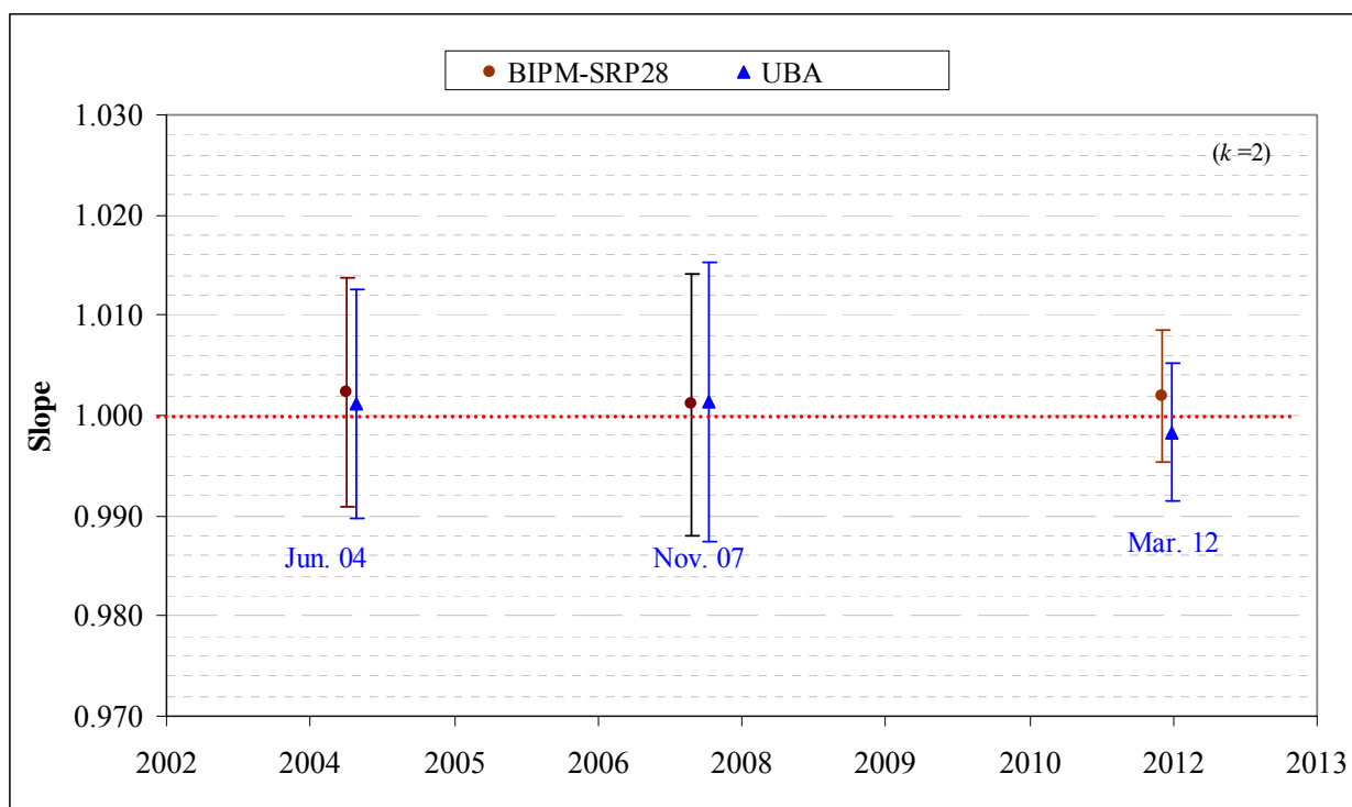
Figure 2 : Results of previous comparisons between SRP27, SRP28 and UBA standards realised at the BIPM. Uncertainties are calculated at k = 2 , with the uncertainty budget in use at the time of each comparison.
