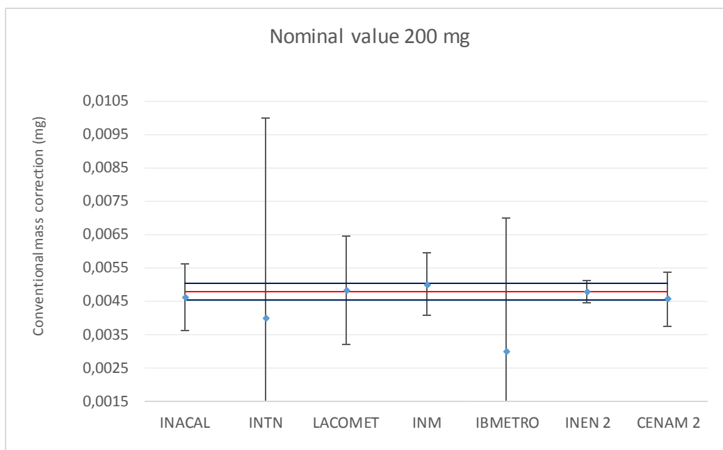
Figure 12. Reported values of conventional mass correction for 200 mg weight by each laboratory. The reference value is represented by the red line and its uncertainty by the blue lines
