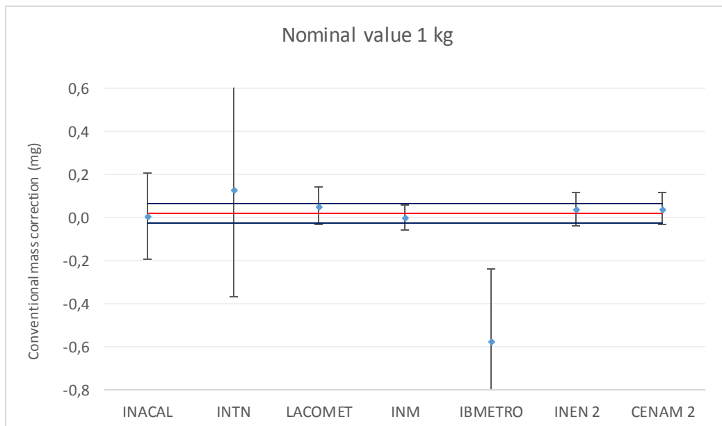
Figure 8. Reported values of conventional mass correction for 1 kg weight by each laboratory. The reference value is represented by the red line and its uncertainty by the blue lines
