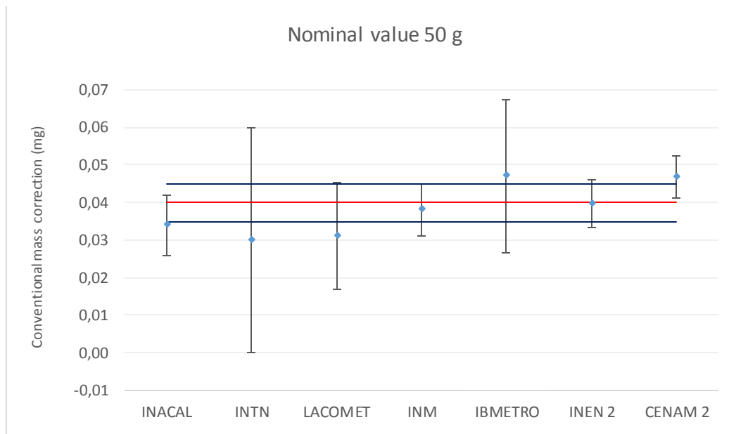
Figure 10. Reported values of conventional mass correction for 50 g weight by each laboratory. The reference value is represented by the red line and its uncertainty by the blue lines
