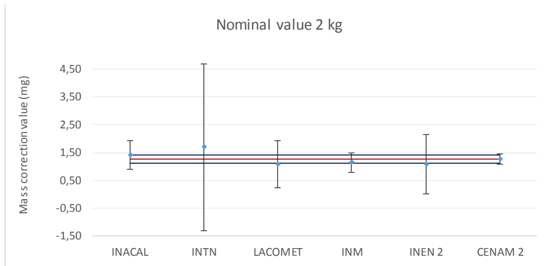
Figure 1. Reported values of mass correction value for 2 kg weight by each laboratory. The reference value is represented by the red line and its uncertainty by the blue lines
