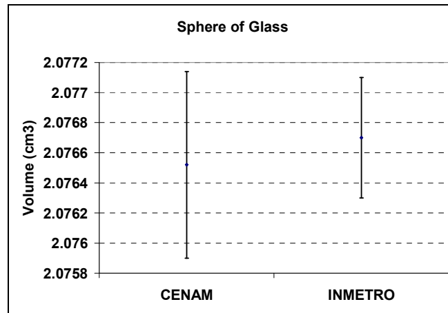
Figure 4. Graph of the volume of the sphere of glass reported by participant laboratories
