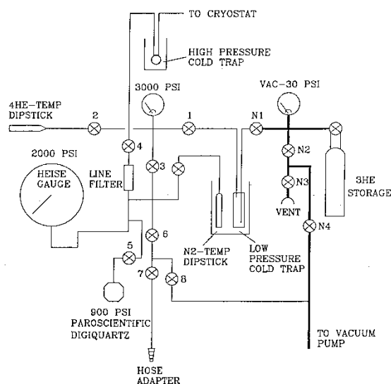
Figure 3. The ^3\text{He} gas-handling system of Adams [2005].
