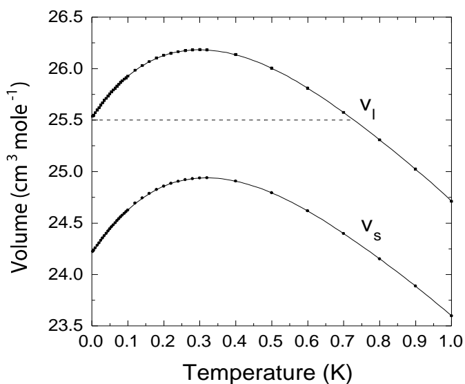
Figure 5. Molar volumes of liquid and solid ^3\text{He} at the melting pressure, with the region of co-existence lying between the two curves, from Adams [2005]. The horizontal dotted line indicates the path taken by the sample if the plug is formed at 3.38 MPa.
