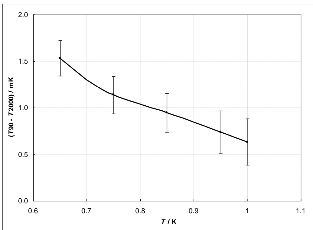
Figure 10. Differences ( T_{90} - T_{2000} ) obtained at PTB from comparisons of ^3\text{He} vapour pressures and melting pressures, using rhodium-iron resistance thermometers as intermediaries [Engert et al. 2007]. Uncertainty bars for the scale comparisons are shown at k = 1 .
