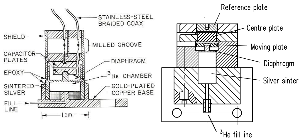
Figure 2. ^3\text{He} melting-pressure cells of Greywall and Busch [1982] (diaphragm of coin silver, diameter 6.4 mm, thickness 0.25 mm) and SHH [Schuster et al. 2001] (diaphragm of BeCu, diameter 6.1 mm, thickness 0.4 mm).
