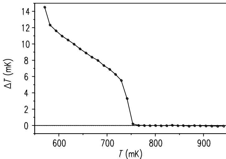
Figure 6. Example of temperature deviations when solid ^3\text{He} is forced to grow into the sinter, from SHH (Figure 14). \Delta T is the difference between the indications of the melting pressure sensor and a reference thermometer on the cell, during cool-down.
