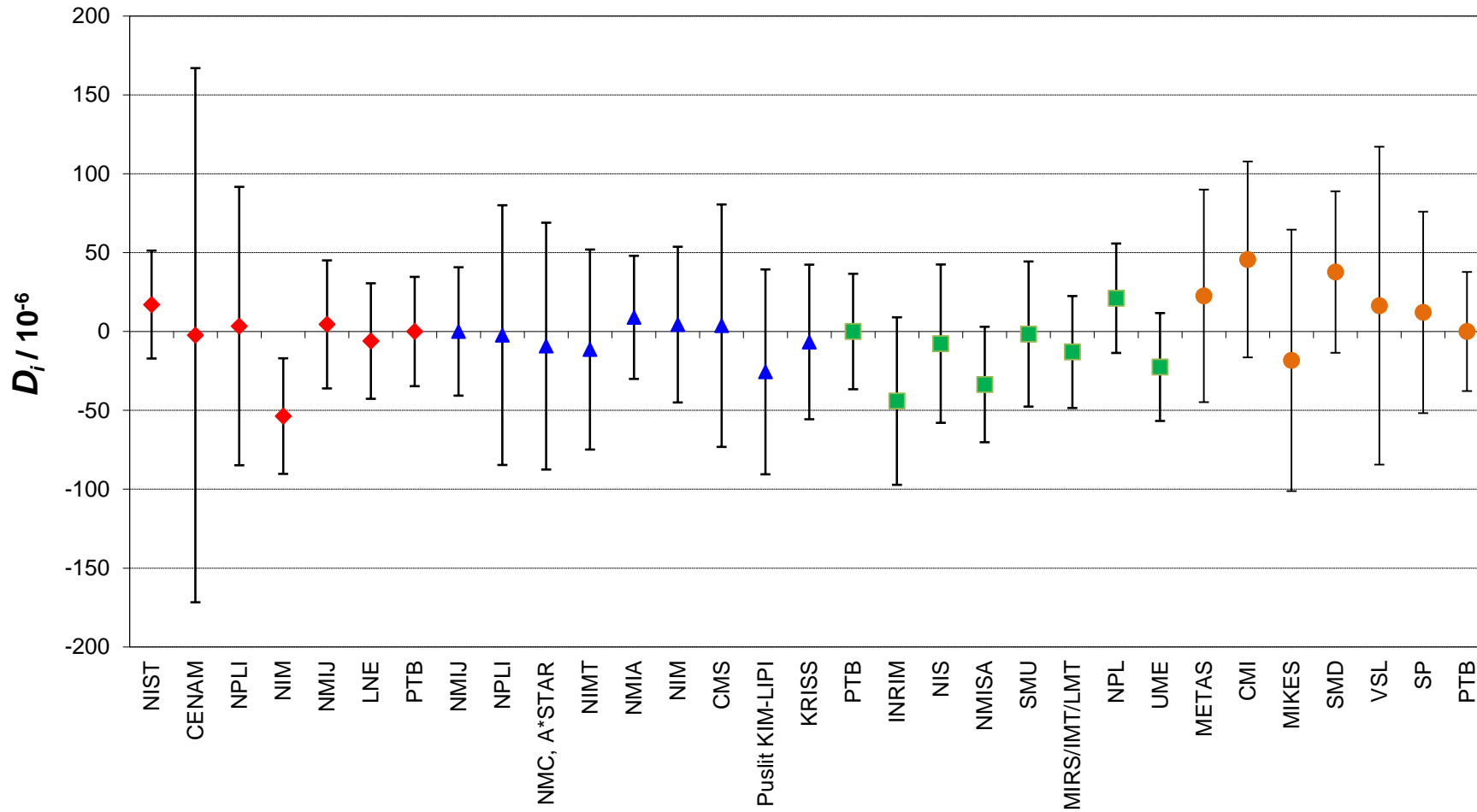
CCM.P-K13, APMP.M.P-K13, EURAMET.M.P-K13 and EURAMET.M.P-K7 200 MPa Degrees of equivalence D_i and U_i ( k = 2 )
