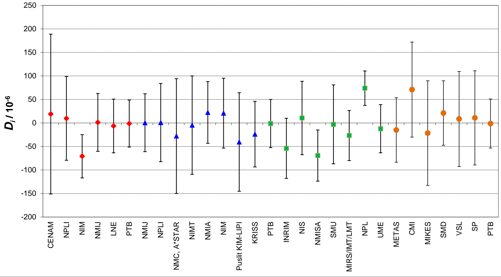
CCM.P-K13, APMP.M.P-K13, EURAMET.M.P-K13 and EURAMET.M.P-K7 400 MPa Degrees of equivalence D_i and U_i ( k = 2 )
