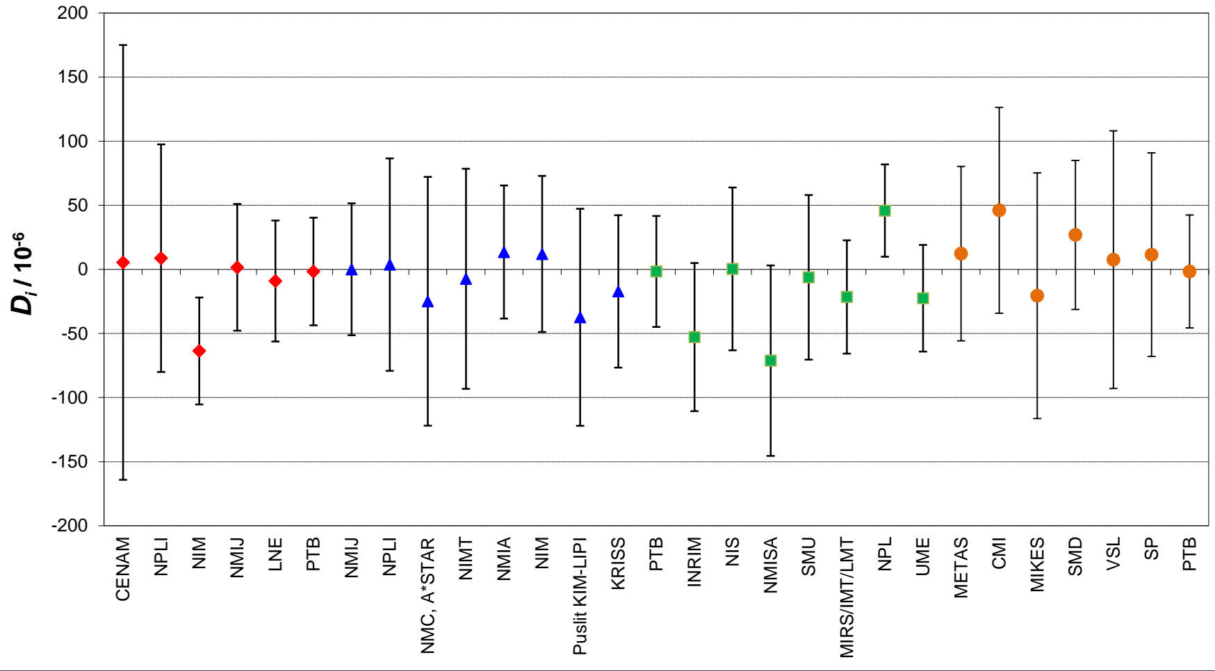
CCM.P-K13, APMP.M.P-K13, EURAMET.M.P-K13 and EURAMET.M.P-K7 300 MPa Degrees of equivalence D_i and U_i ( k = 2 )
