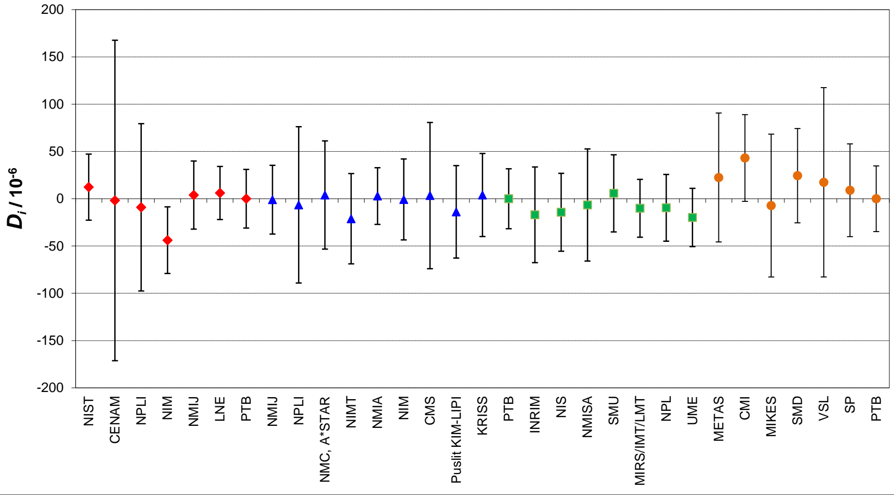
CCM.P-K13, APMP.M.P-K13, EURAMET.M.P-K13 and EURAMET.M.P-K7 100 MPa Degrees of equivalence D_i and U_i ( k = 2 )
