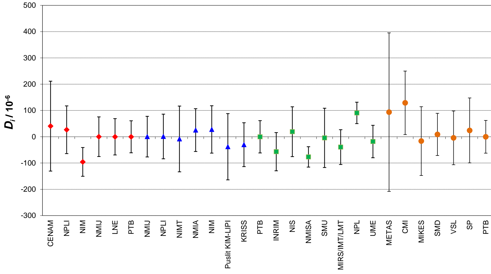
CCM.P-K13, APMP.M.P-K13, EURAMET.M.P-K13 and EURAMET.M.P-K7 500 MPa Degrees of equivalence D_i and U_i ( k = 2 )
