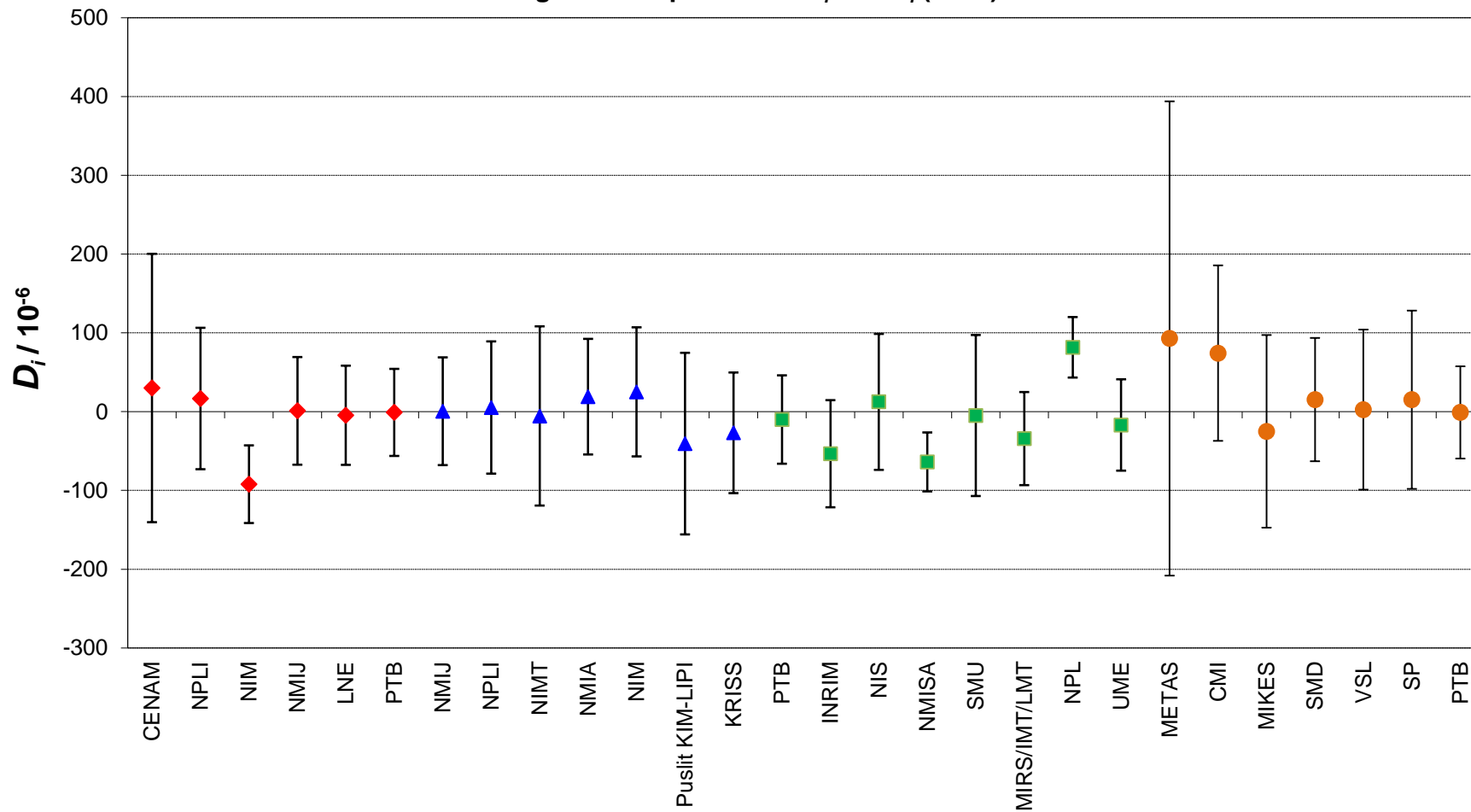
CCM.P-K13, APMP.M.P-K13, EURAMET.M.P-K13 and EURAMET.M.P-K7 450 MPa Degrees of equivalence D_i and U_i ( k = 2 )
