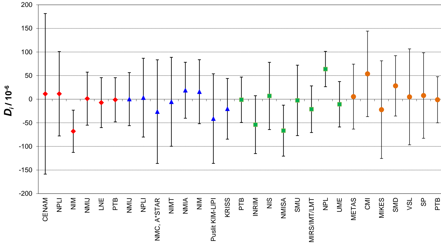
CCM.P-K13, APMP.M.P-K13, EURAMET.M.P-K13 and EURAMET.M.P-K7 350 MPa Degrees of equivalence D_i and U_i ( k = 2 )
