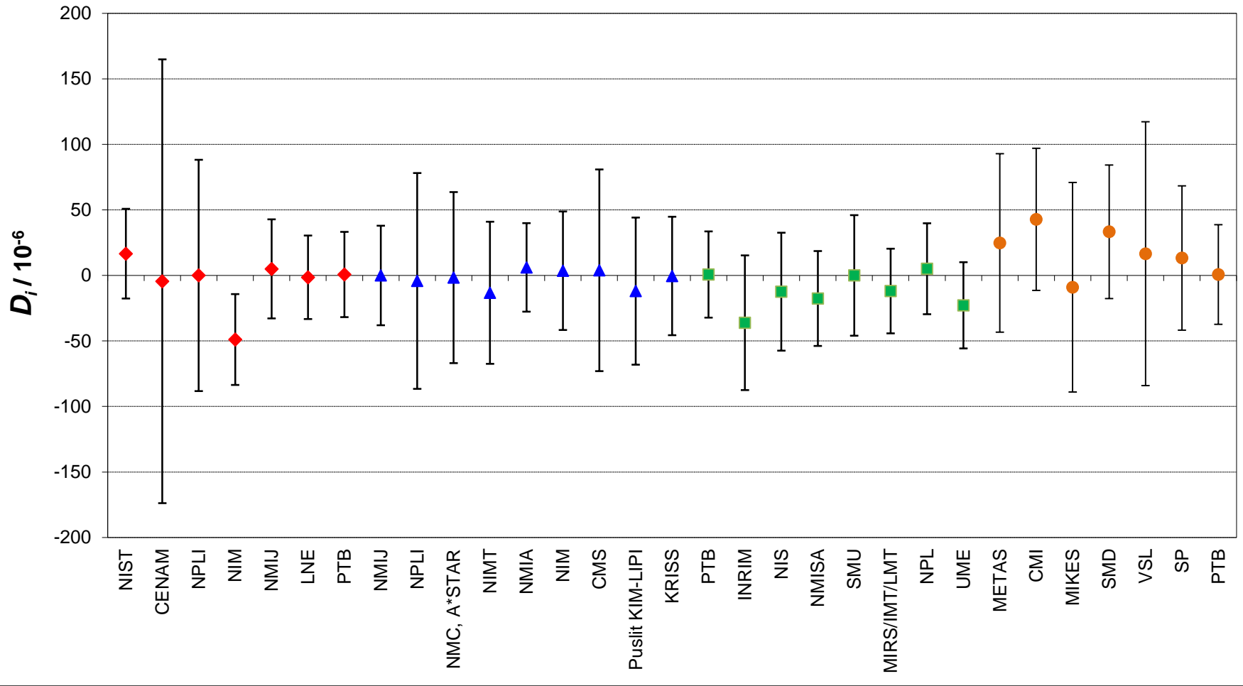
CCM.P-K13, APMP.M.P-K13, EURAMET.M.P-K13 and EURAMET.M.P-K7 150 MPa Degrees of equivalence D_i and U_i ( k = 2 )
