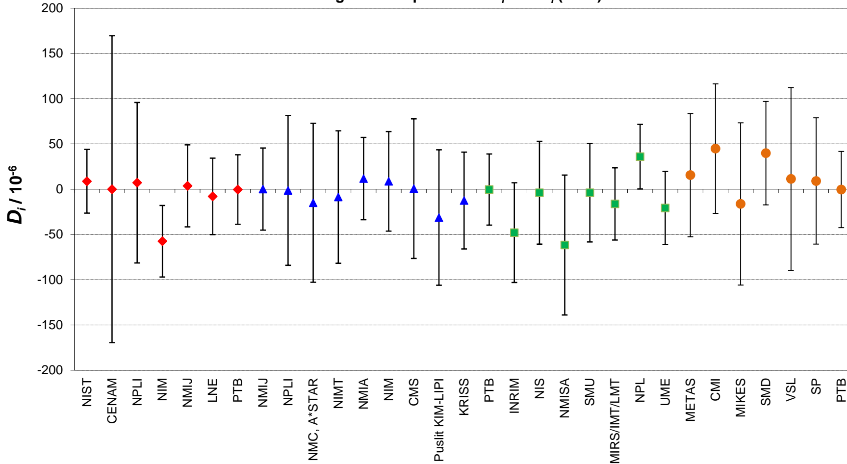
CCM.P-K13, APMP.M.P-K13 , EURAMET.M.P-K13 and EURAMET.M.P-K7 250 MPa Degrees of equivalence D_i and U_i ( k = 2 )
