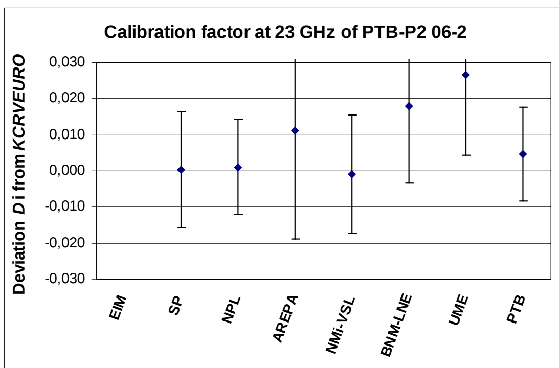
Fig. 5.6 b Deviation D_i of the measured calibration factor K(f) from the KCRVEURO at 23 GHz with expanded uncertainty bars ( k=2 ) for PTB-P2 06-2
