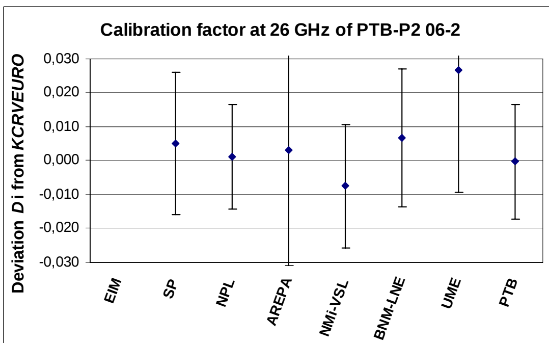
Fig. 5.7 b Deviation D_i of the measured calibration factor K(f) from the KCRVEURO at 26 GHz with expanded uncertainty bars ( k=2 ) for PTB-P2 06-2
