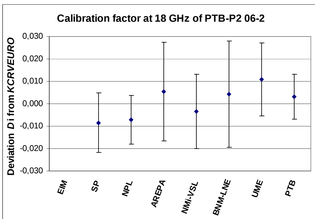
Fig. 5.4 b Deviation D_i of the measured calibration factor K(f) from the K_{CRVEURO} at 18 GHz with expanded uncertainty bars ( k=2 ) for PTB-P2 06-2
