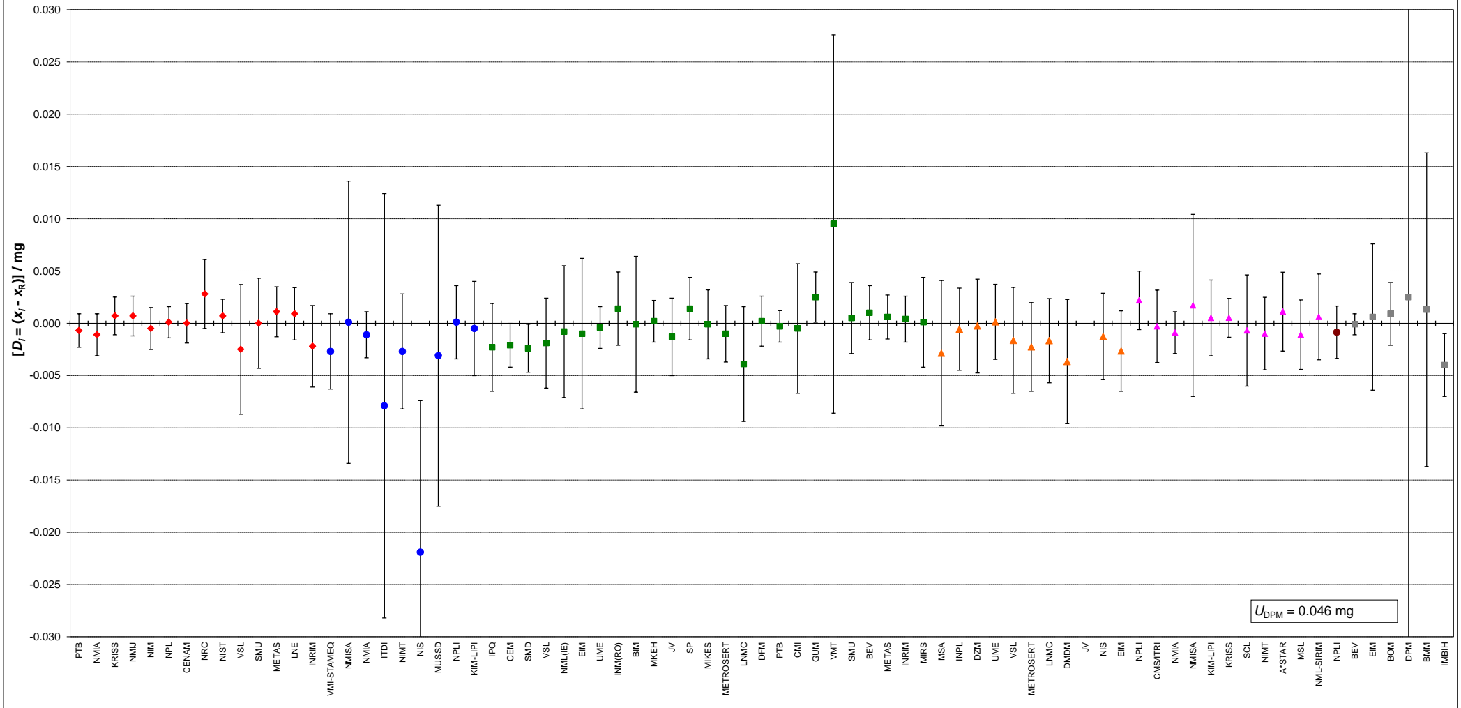
CCM.M-K2 , APMP.M.M-K6, EUROMET.M.M-K2, EUROMET.M.M-K2.1, APMP.M.M-K2&K2.1, and EURAMET.M.M-K2.2 2 g mass standards Degrees of equivalence: D_i and expanded uncertainty U_i
