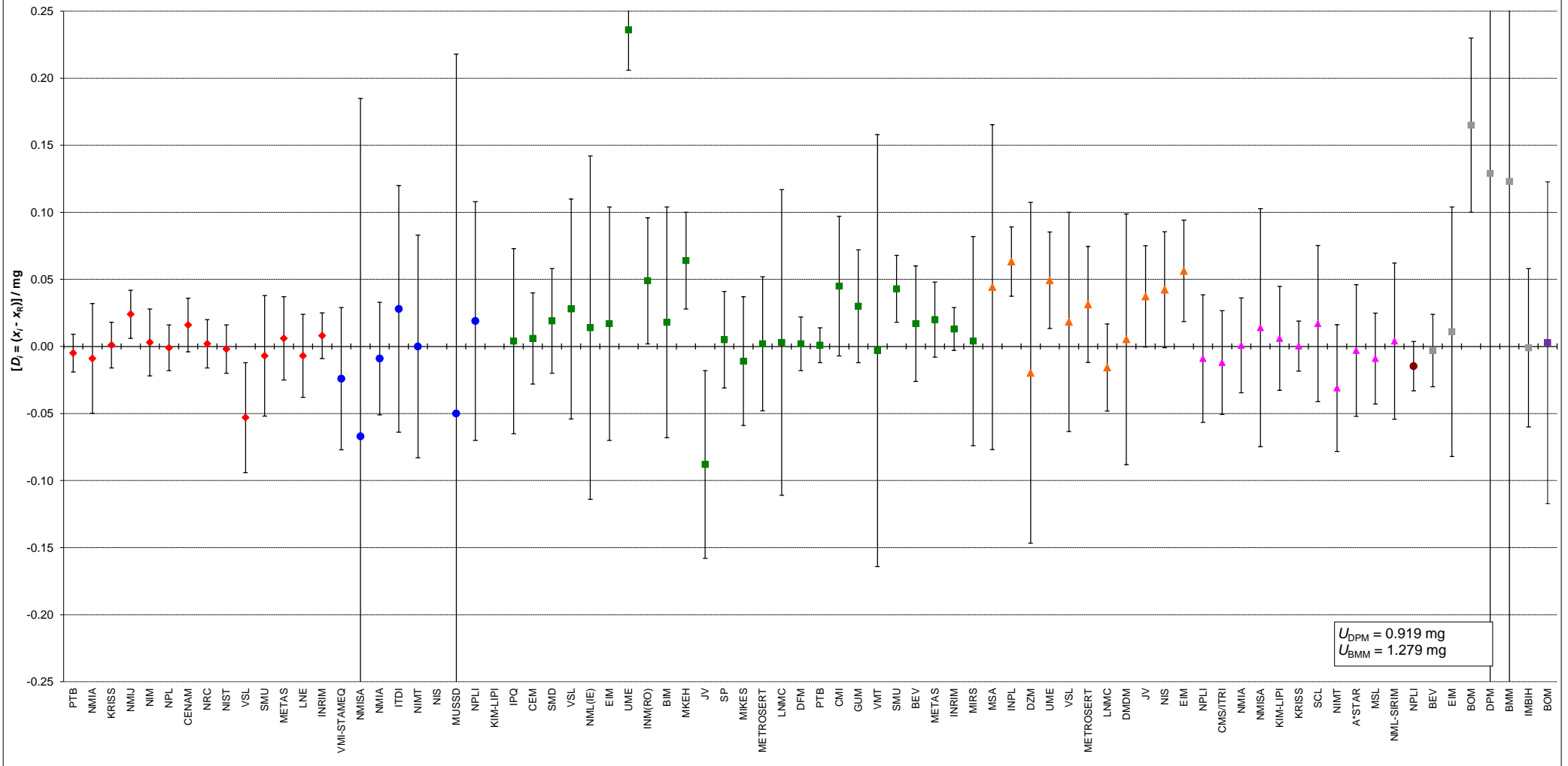
CCM.M-K2 , APMP.M.M-K6, EUROMET.M.M-K2, EUROMET.M.M-K2.1, APMP.M.M-K2&K2.1, EURAMET.M.M-K2.2, and EURAMET.M.M-K2.3 500 g mass standards Degrees of equivalence: D_i and expanded uncertainty U_i
