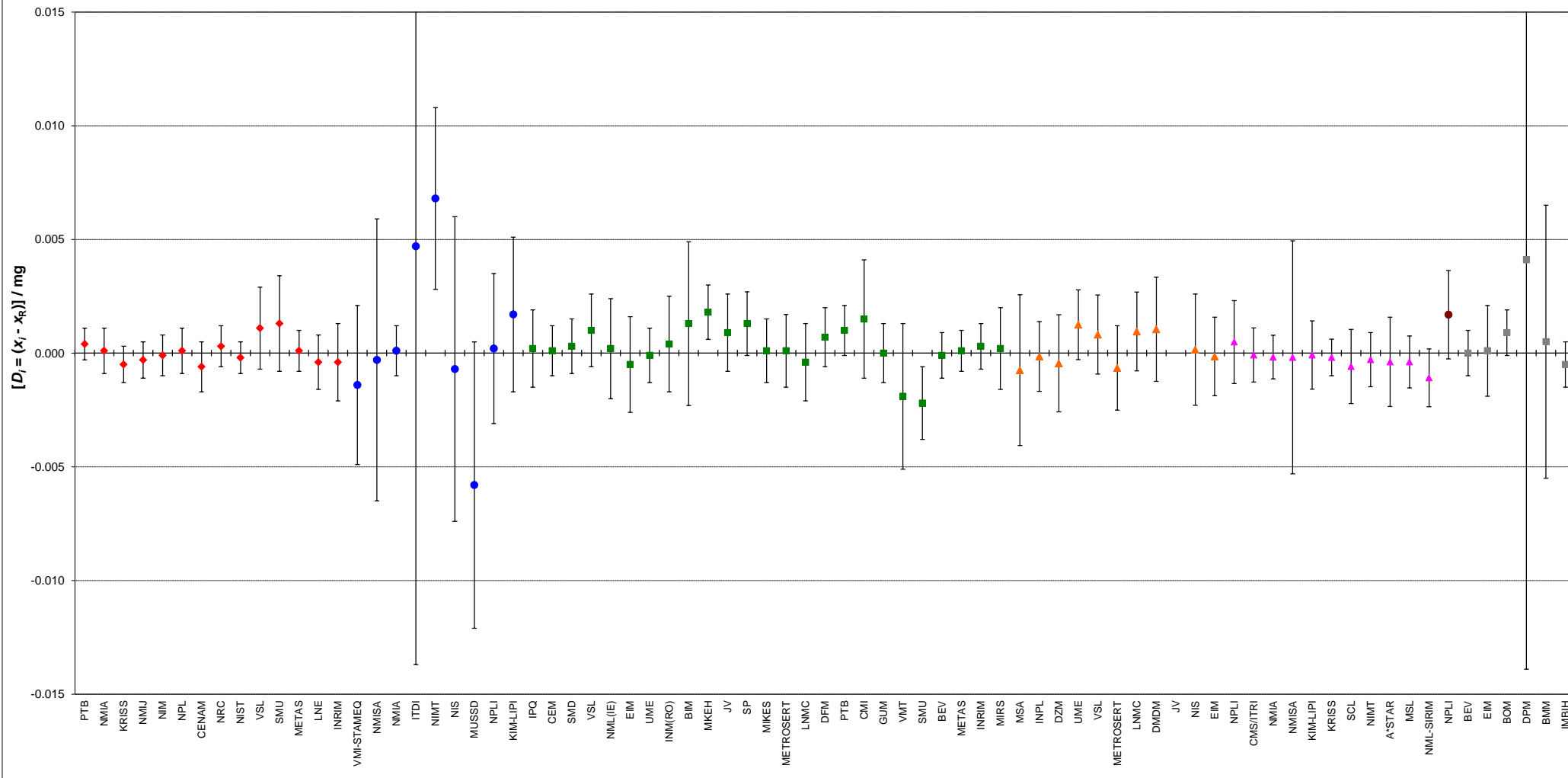
CCM.M-K2 , APMP.M-M-K6, EUROMET.M-M-K2, EUROMET.M-M-K2.1, APMP.M-M-K2&K2.1, and EURAMET.M-M-K2.2 100 mg mass standards Degrees of equivalence: D_i and expanded uncertainty U_i
