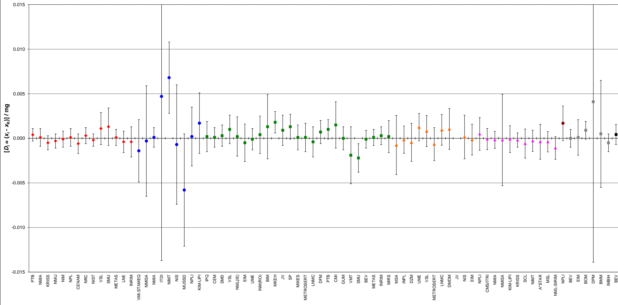
CCM.M-K2 , APMP.M.M-K6, EUROMET.M.M-K2, EUROMET.M.M-K2.1, APMP.M.M-K2&K2.1, and EURAMET.M.M-K2.2&K2.6 100 mg mass standards Degrees of equivalence: D_i and expanded uncertainty U_i
