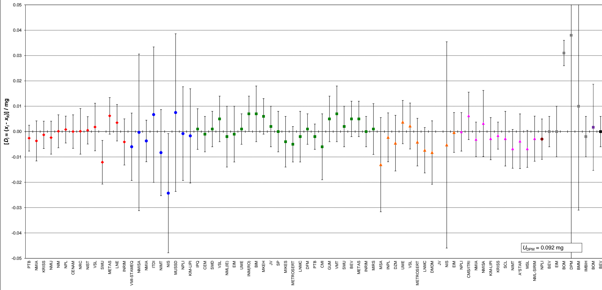
CCM.M-K2, APMP.M.M-K6, EUROMET.M.M-K2&K2.1, APMP.M.M-K2&K2.1, EURAMET.M.M-K2.2,K2.3&K2.6 20 g mass standards Degrees of equivalence: D_i and expanded uncertainty U_i
