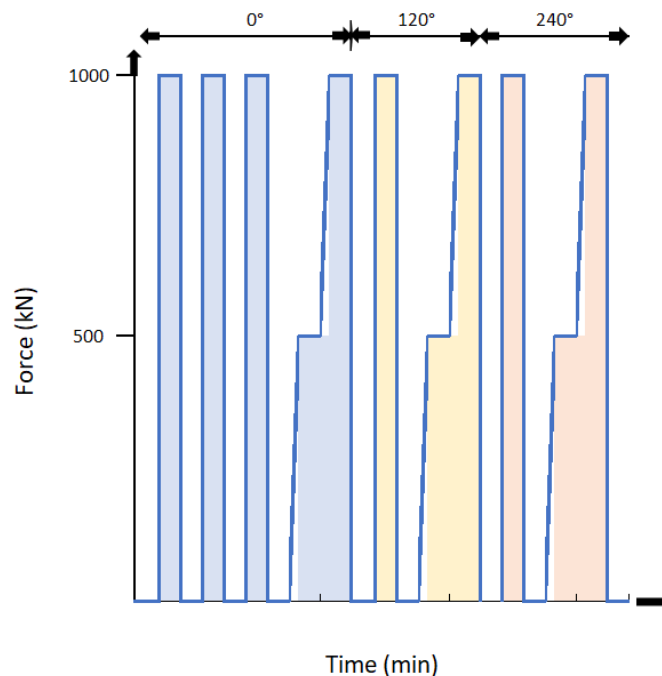
Illustration 1. Measurement scheme
