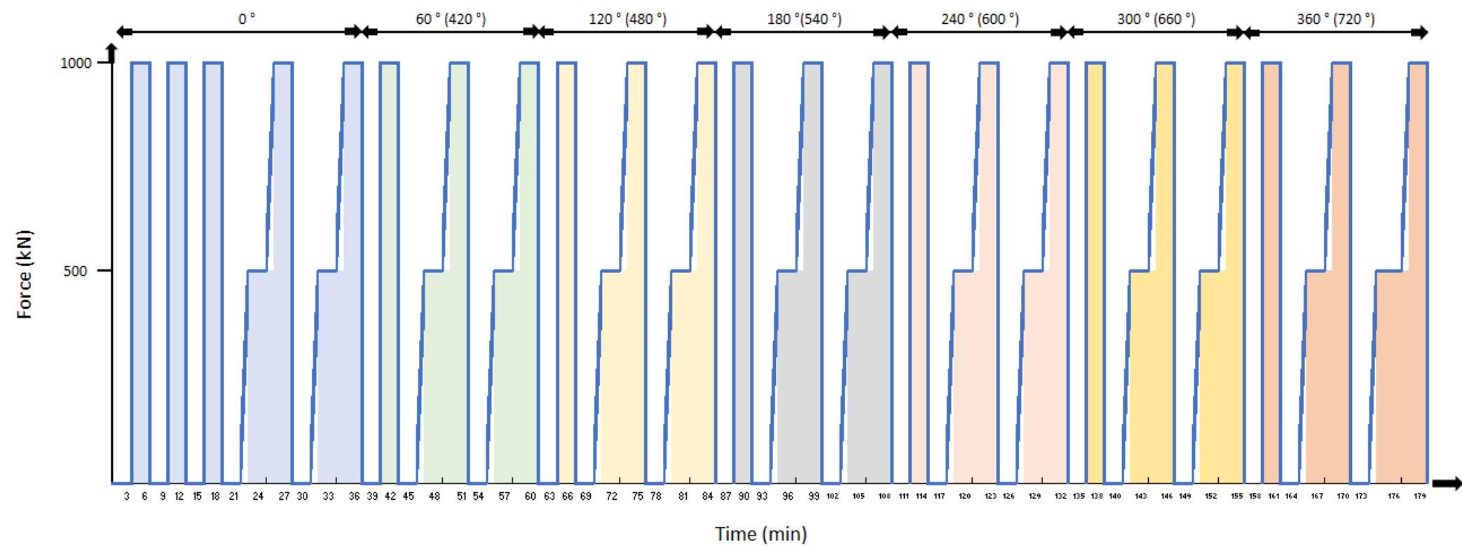
Figure 2. Measurement sequence
