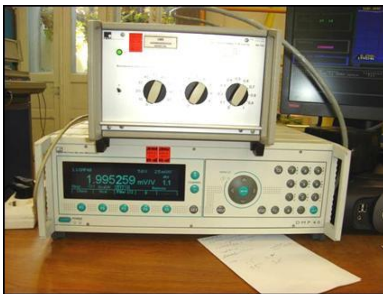
Figure 1. Precision indicating instrument (DMP 40) and BN 100 calibrator of TÜBİTAK UME
