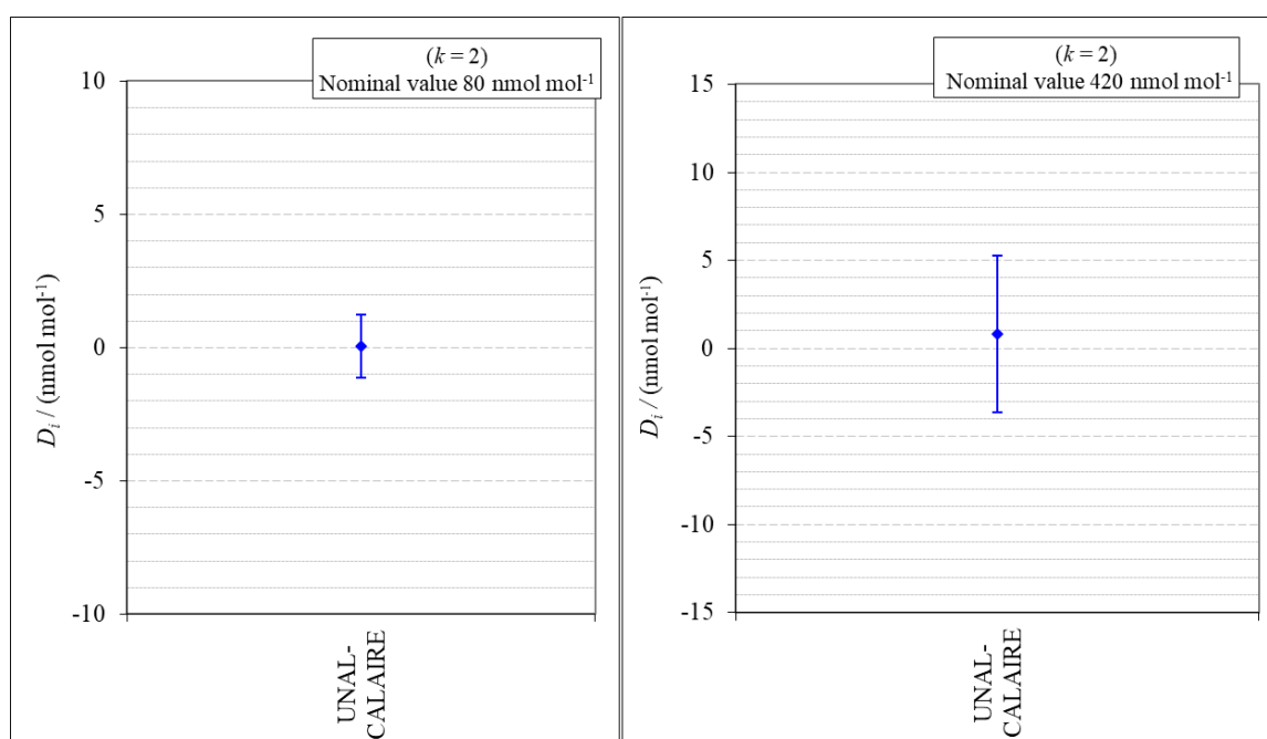
Figure 1: Degrees of equivalence of the UNAL-CALAIRE at the two nominal ozone amount fractions 80 nmol mol -1 and 420 nmol mol -1
