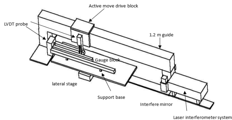
Fig. 1 Illustration of long gauge block calibration system
