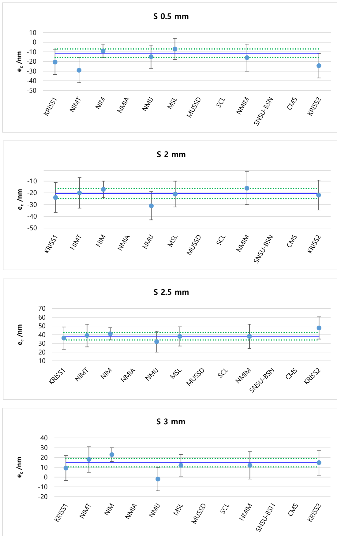
Figure 8. Measurement results and KCRV for short gauge blocks.
