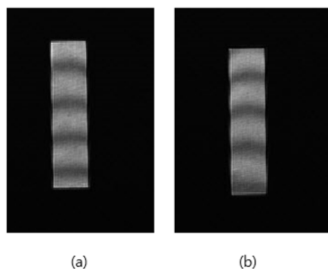
Figure 3 – Interferograms (provided by NIMT) of the two measuring faces of the 400 mm long gauge block
