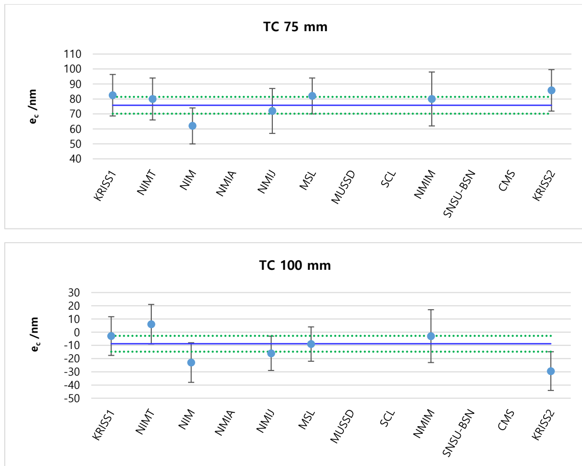
Figure 8. Measurement results and KCRV for short gauge blocks (continued).
