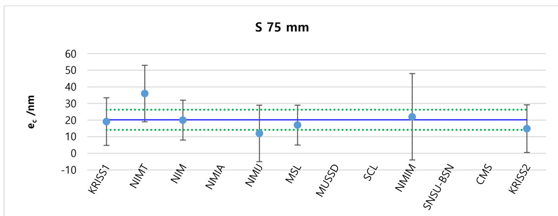
Figure 8. Measurement results and KCRV for short gauge blocks (continued).
