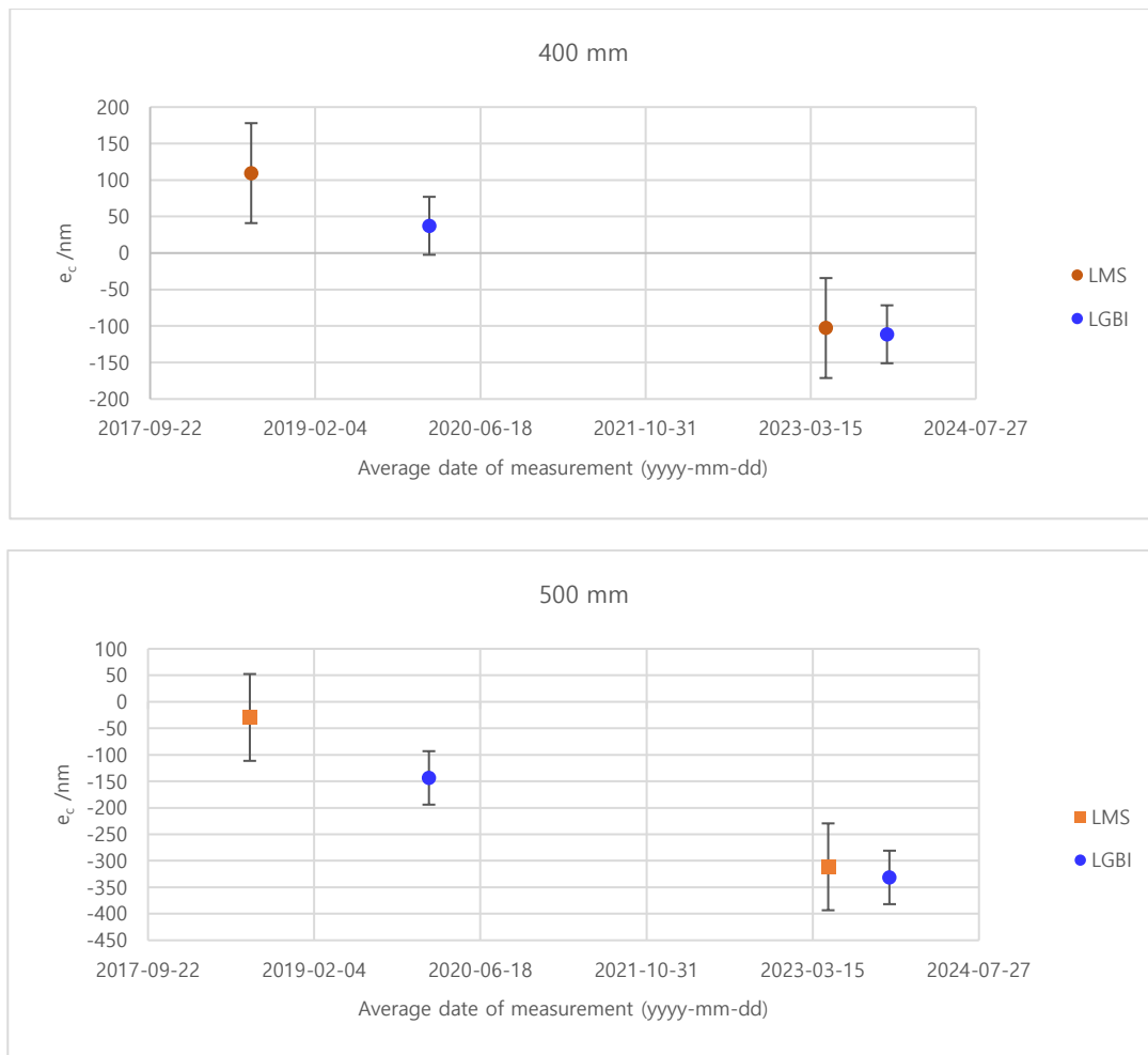
Figure 1. Measurement results of two long gauge blocks by pilot lab using a linear measuring system (LMS, brown squares) and long gauge block interferometer (LGBI, blue dots) before and after the circulation of artefacts. The uncertainty bar shows standard uncertainty ( k=1 ).
