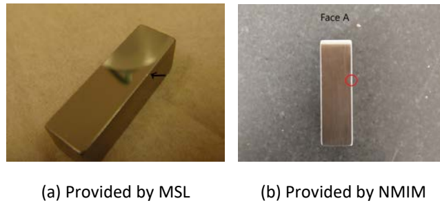
Figure 4 – Photos of the 10 mm steel gauge block showing a dent on the edge of face A.
