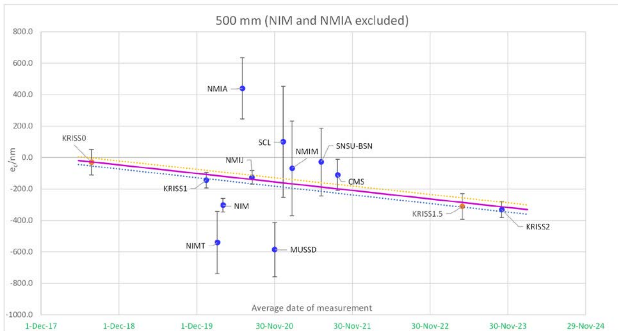
Figure 14. Measurement results and KCRV for 500 mm long gauge block (-results of NIM and NMIA excluded). Dotted lines represent the standard uncertainty of KCRV. Orange dots labeled as KRISS0 and KRISS1.5 are results of pilot obtained with LMS, but are not used for the KCRV calculation.
