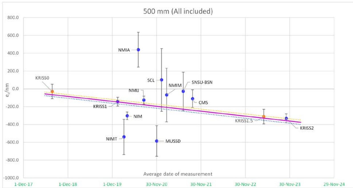
Figure 12. Measurement results and KCRV for 500 mm long gauge block (- all participants included). Dotted lines represent the standard uncertainty of KCRV. Orange dots labeled as KRISO and KRISS1.5 are results of pilot obtained with LMS, but are not used for KCRV calculation.
