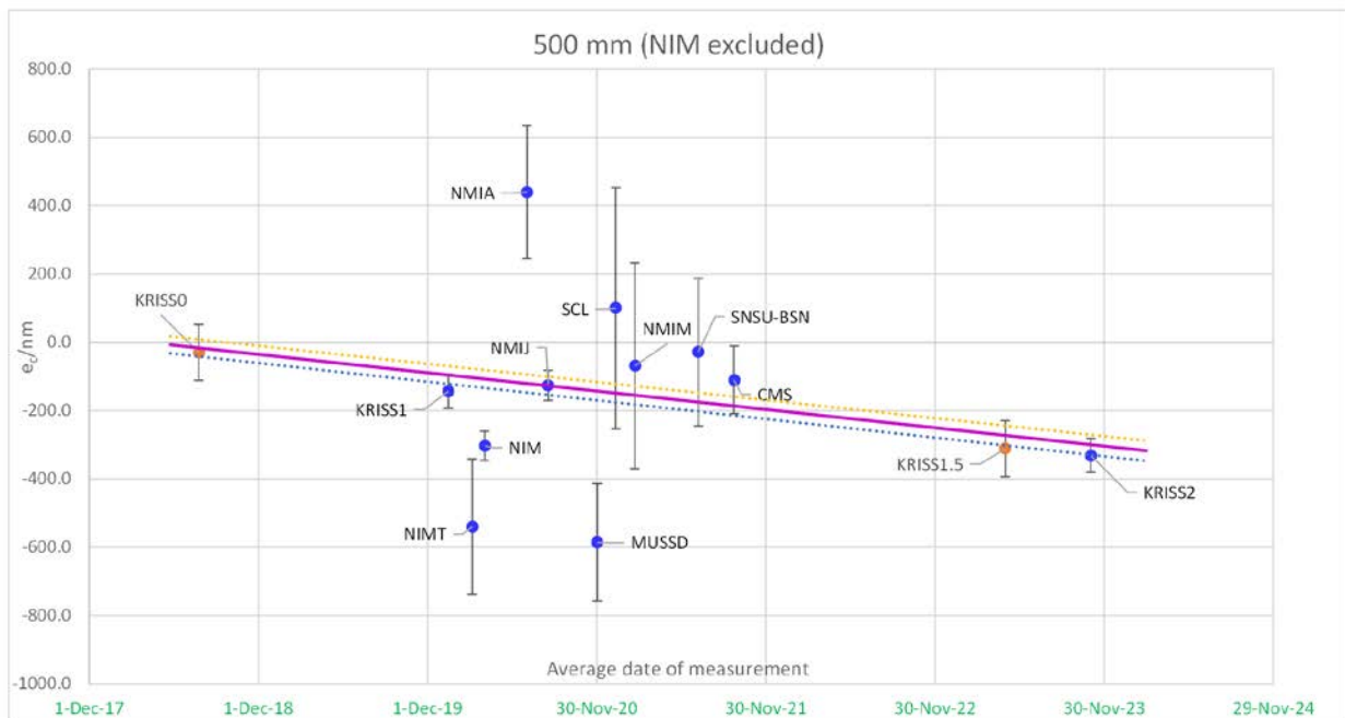
Figure 13. Measurement results and KCRV for 500 mm long gauge block (- NIM’s result excluded). Dotted lines represent the standard uncertainty of KCRV. Orange dots labeled as KRISS0 and KRISS1.5 are results of pilot obtained with LMS, but are not used for KCRV calculation.
