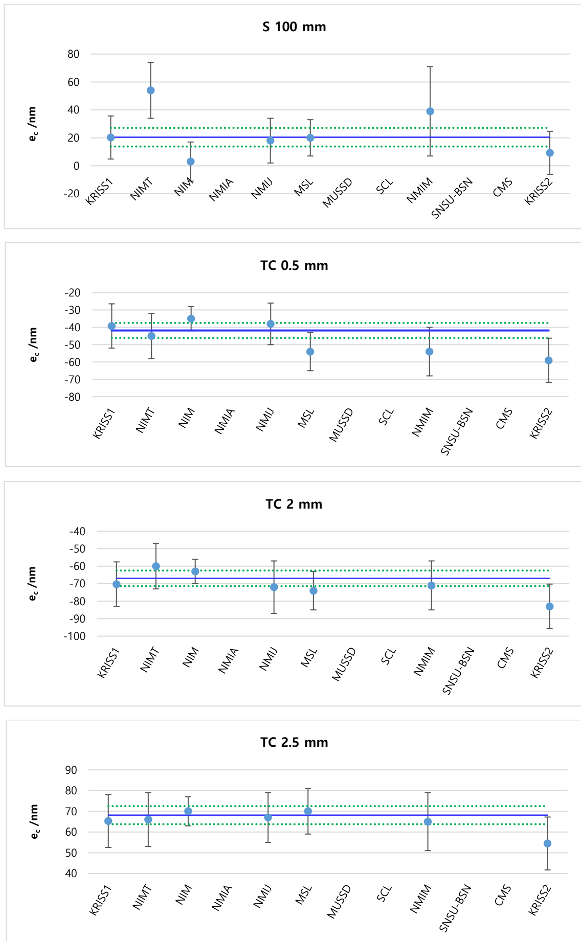
Figure 8. Measurement results and KCRV for short gauge blocks (continued).
