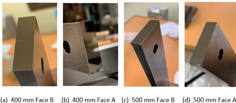
Figure 6 – Photo (provided by SCL) of scratches on measuring faces of long gauge blocks
