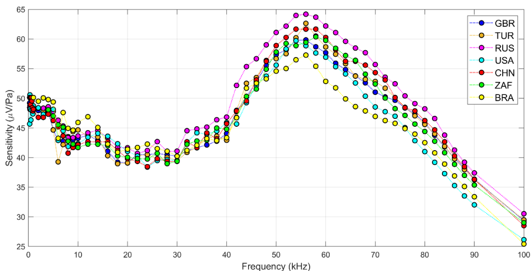
Figure 5.3 The reported linear sensitivities for the B&K8104 hydrophone from 250 Hz to 100 kHz.
