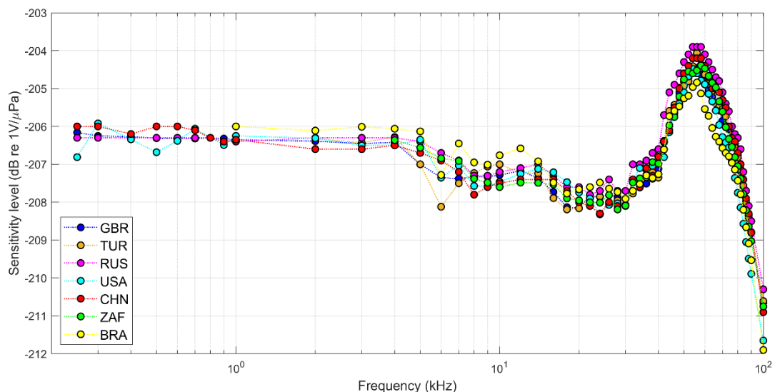
Figure 5.2 The reported sensitivity levels for the B&K8104 hydrophone from 250 Hz to 100 kHz (log frequency scale).
