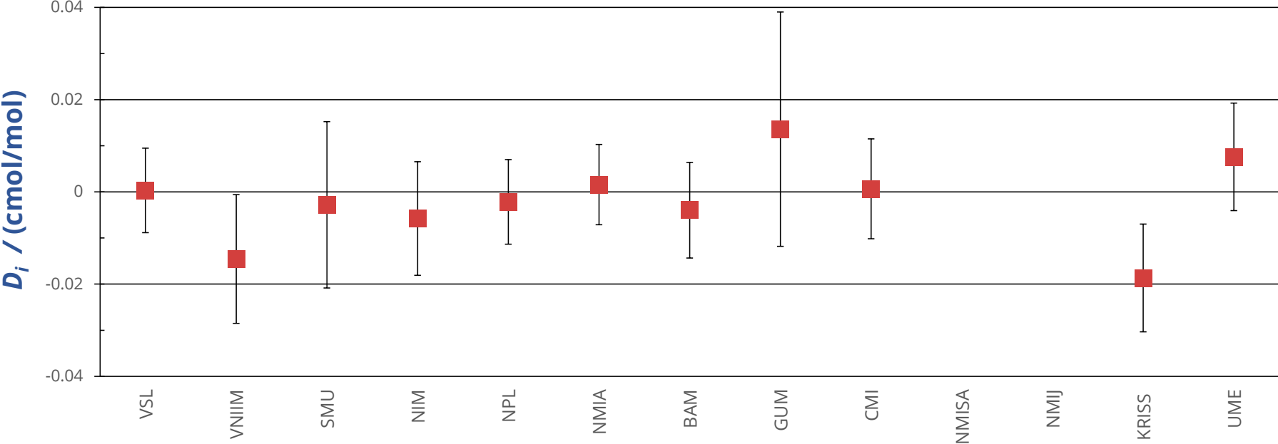
CCQM-K118, CO2 in low calorific gas
