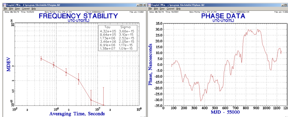
Figure 1. UTC – UTC(TL), stability and phase difference
