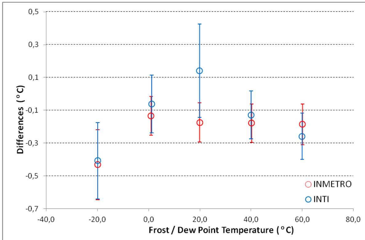
Figure 4 – Measurement Differences and associated Expanded Uncertainty
