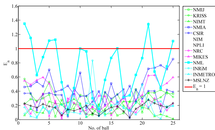
Fig. 10-3 E_n numbers calculated except NPLI and NIM
