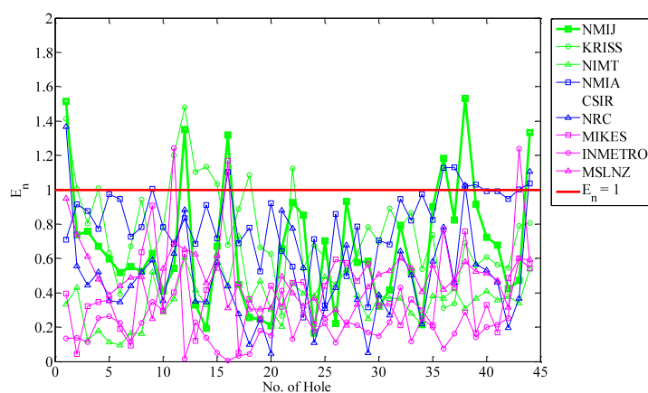
Fig. 10-19 E_n numbers calculated except CSIR
