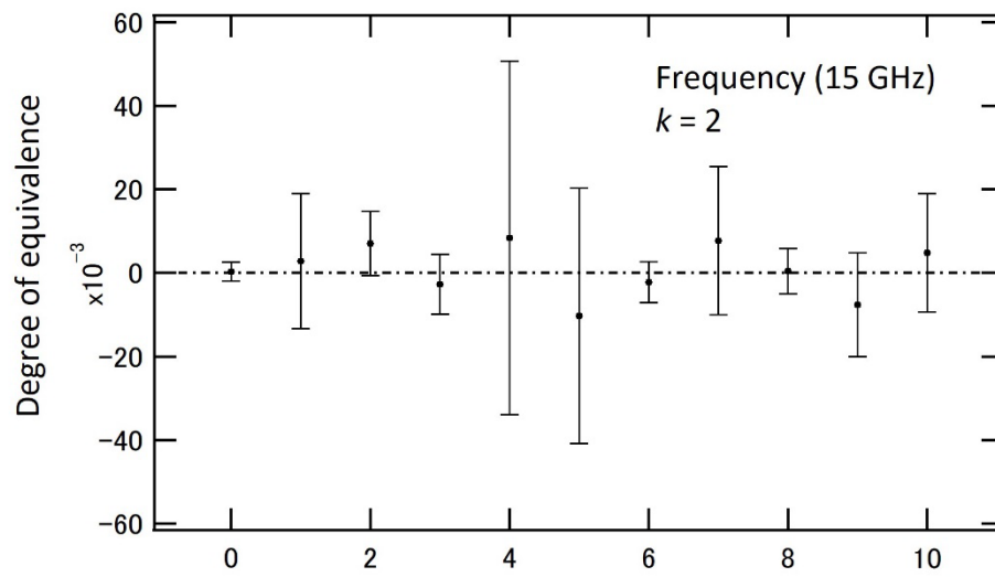
Fig. 8.14 DoE between m(L_i) and APMP RV (15 GHz, Sensor No. 2)
