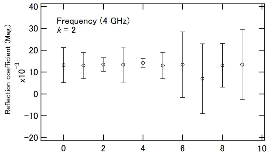
Fig. A.8 Reflection coefficient (4 GHz, Sensor No.2)
