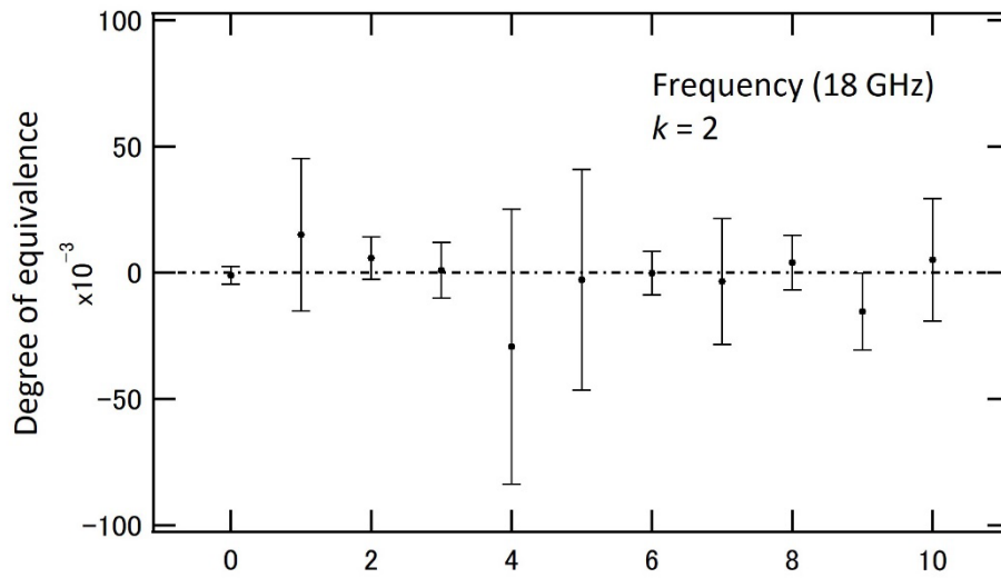
Fig. 8.15 DoE between m(L_i) and APMP RV (18 GHz, Sensor No. 1)
