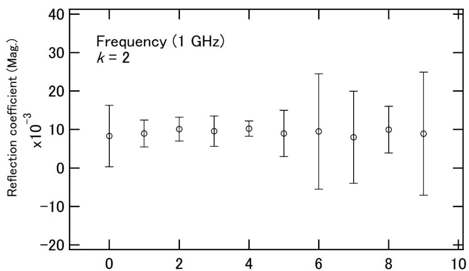
Fig. A.6 Reflection coefficient (1 GHz, Sensor No.2)
