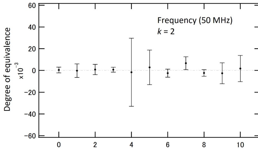
Fig. 8.3 DoE between m(L_i) and APMP RV (50 MHz, Sensor No. 1)
