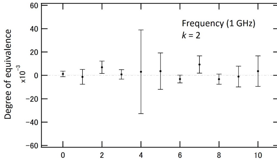
Fig. 8.6 DoE between m(L_i) and APMP RV (1 GHz, Sensor No. 2)
