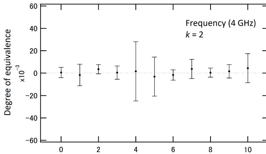
Fig. 9.4 DoE between m(L_i) and CCEM KCRV (4 GHz)
