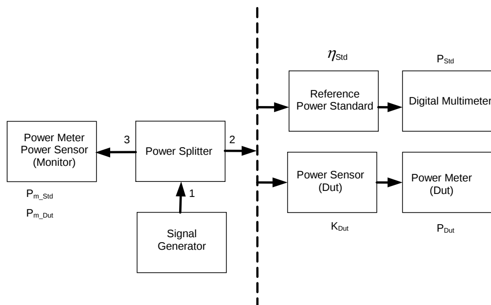
Direct Comparison System Setup
