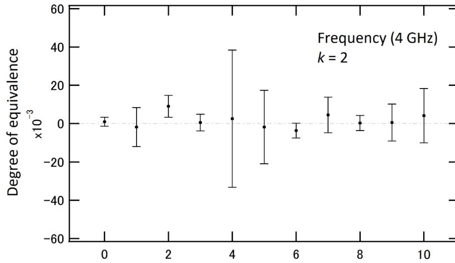
Fig. 8.8 DoE between m(L_i) and APMP RV (4 GHz, Sensor No. 2)
