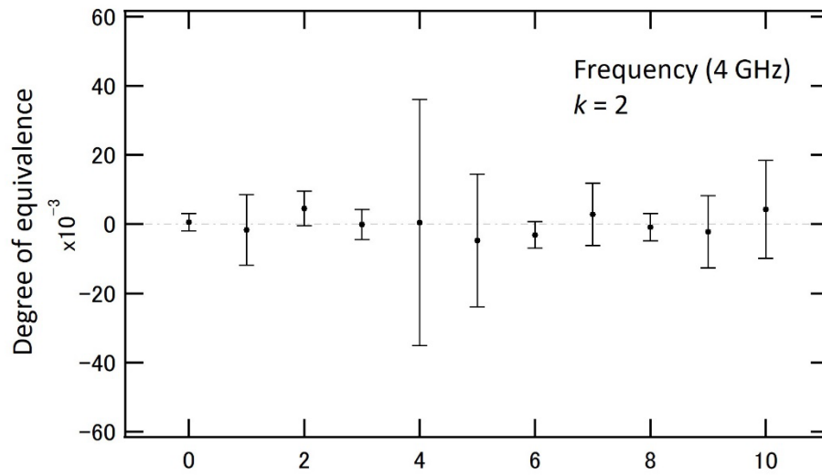
Fig. 8.7 DoE between m(L_i) and APMP RV (4 GHz, Sensor No. 1)
