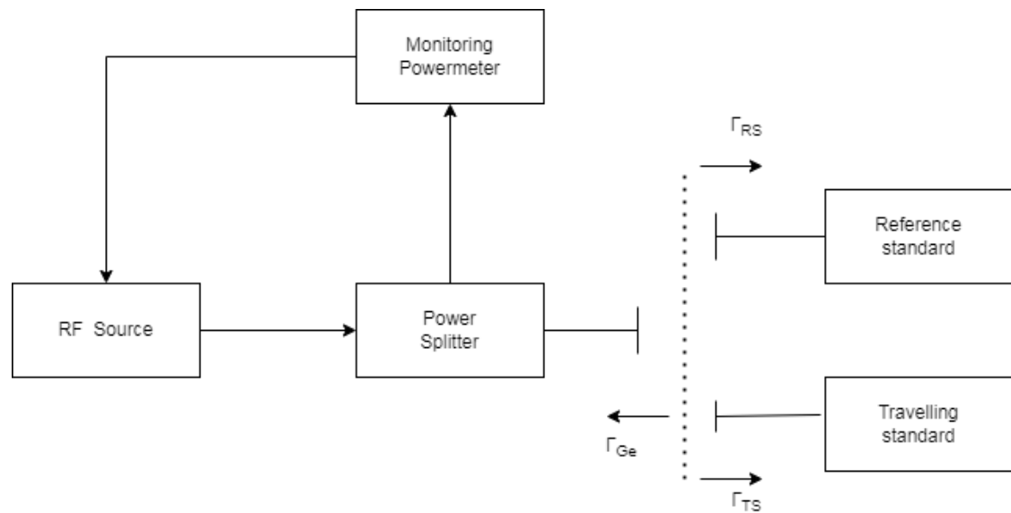
Fig.1 (0.01~18) GHz Type N Connector RF Power Transfer System
