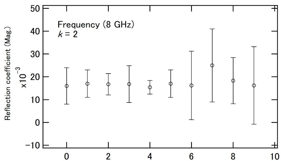
Fig. A.10 Reflection coefficient (8 GHz, Sensor No.2)
