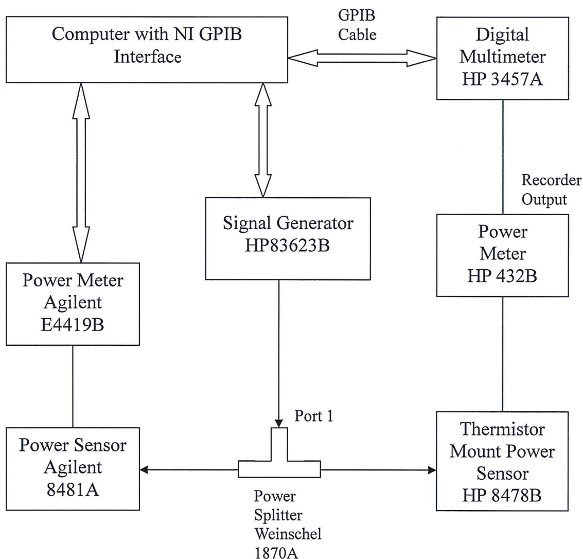
Figure 1 – Measurement Set Up Diagram
