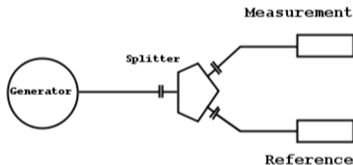
Figure 1: Measurement setup showing sensors connected to the reference and measurement ports.
