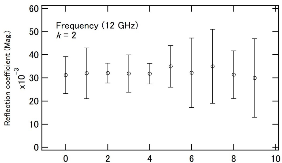
Fig. A.12 Reflection coefficient (12 GHz, Sensor No.2)
