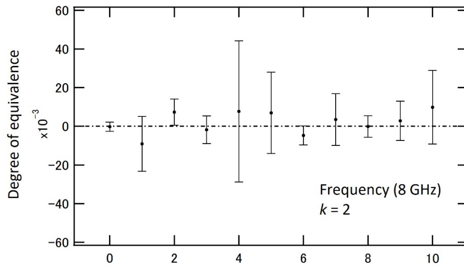
Fig. 8.10 DoE between m(L_i) and APMP RV (8 GHz, Sensor No. 2)
