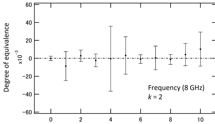
Fig. 8.9 DoE between m(L_i) and APMP RV (8 GHz, Sensor No. 1)
