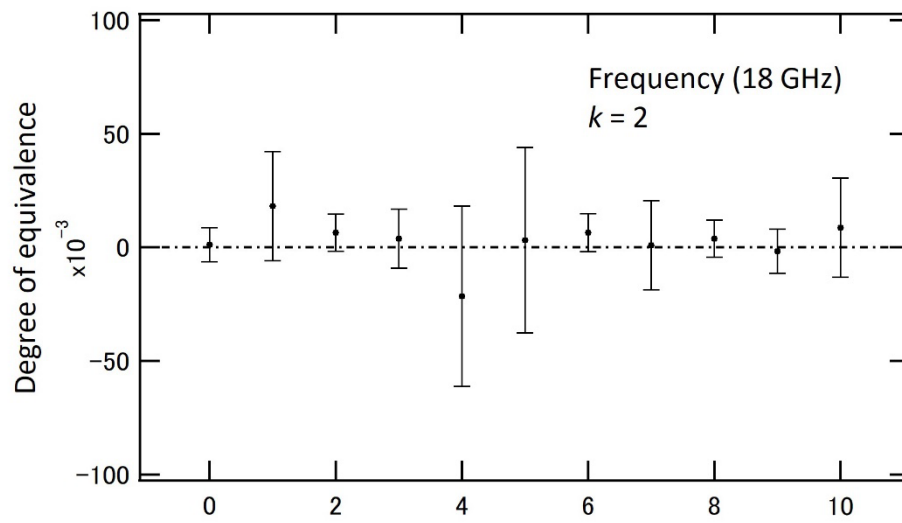
Fig. 9.8 DoE between m(L_i) and CCEM KCRV (18 GHz)
