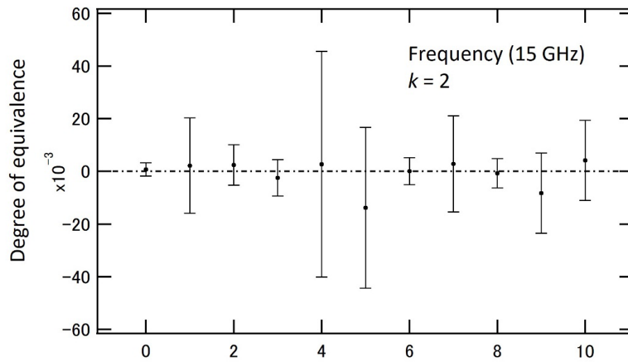
Fig. 8.13 DoE between m(L_i) and APMP RV (15 GHz, Sensor No. 1)
