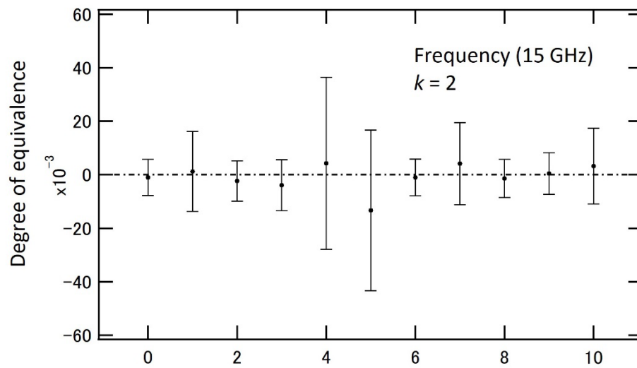
Fig. 9.7 DoE between m(L_i) and CCEM KCRV (15 GHz)
