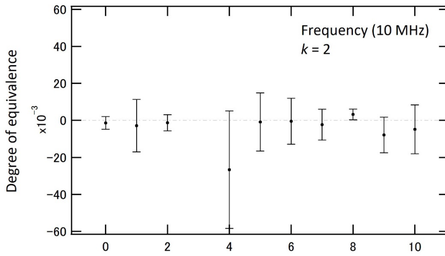
Fig. 8.1 DoE between m(L_i) and APMP RV (10 MHz, Sensor No. 1)
