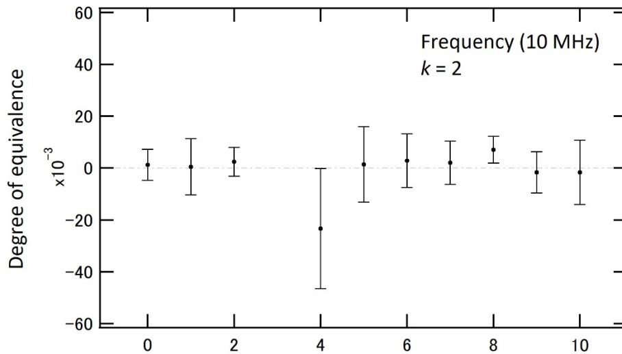
Fig. 9.1 DoE between m(L_i) and CCEM KCRV (10 MHz)
