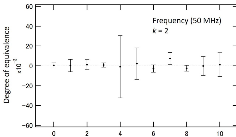
Fig. 8.4 DoE between m(L_i) and APMP RV (50 MHz, Sensor No. 2)
