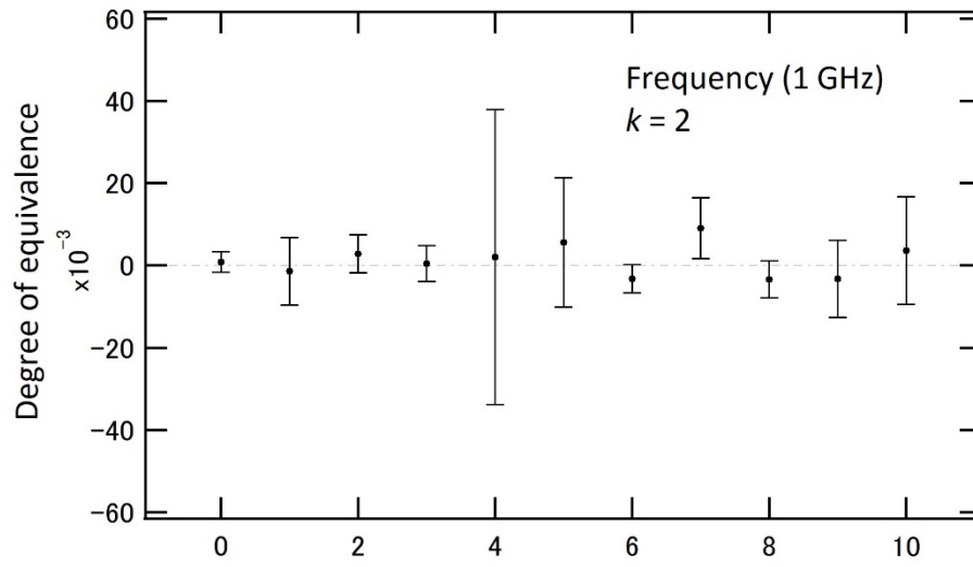
Fig. 8.5 DoE between m(L_i) and APMP RV (1 GHz, Sensor No. 1)
