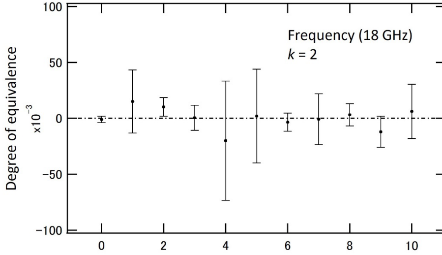
Fig. 8.16 DoE between m(L_i) and APMP RV (18 GHz, Sensor No. 2)
