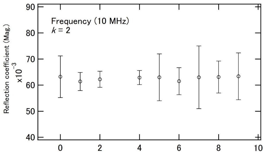
Fig. A.2 Reflection coefficient (10 MHz, Sensor No.2)
