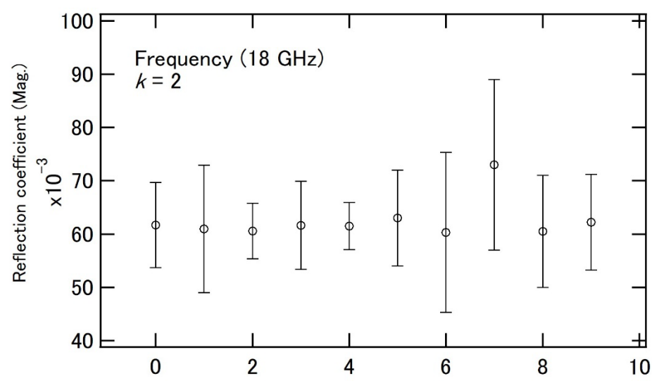
Fig. A.16 Reflection coefficient (18 GHz, Sensor No.2)
