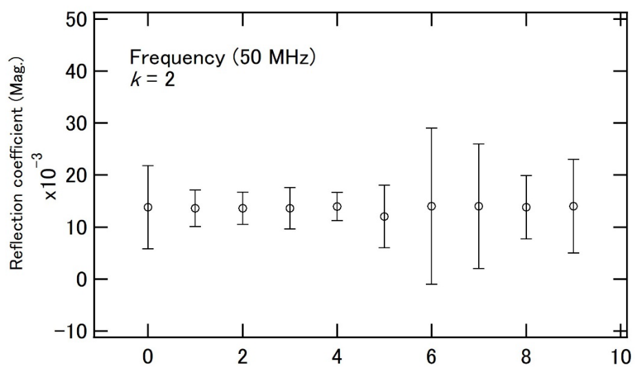
Fig. A.4 Reflection coefficient (50 MHz, Sensor No.2)
