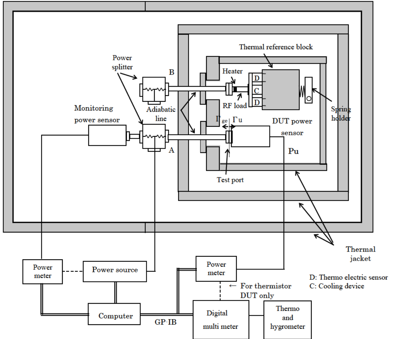
Fig. 1 7 mm coaxial calorimeter, comparison calibration mode
