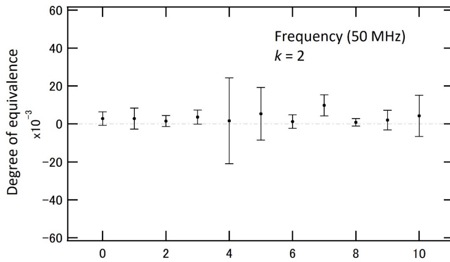
Fig. 9.2 DoE between m(L_i) and CCEM KCRV (50 MHz)
