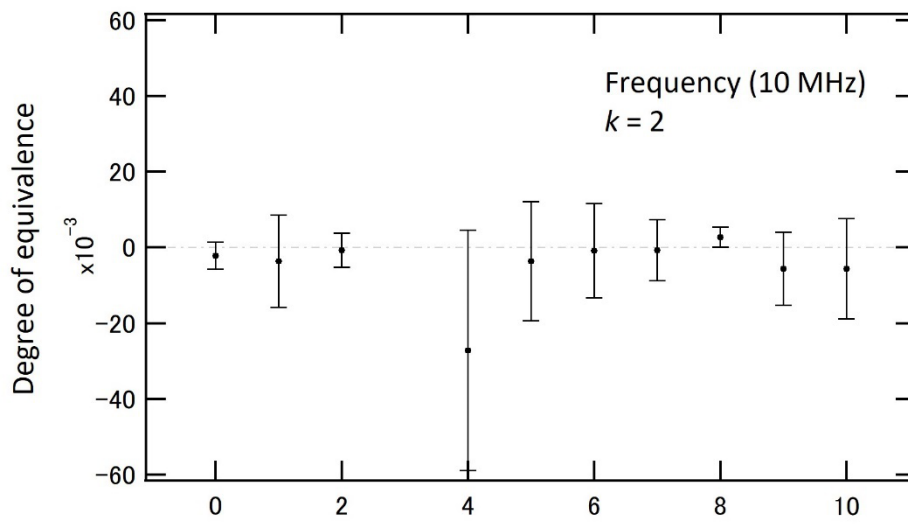
Fig. 8.2 DoE between m(L_i) and APMP RV (10 MHz, Sensor No. 2)
