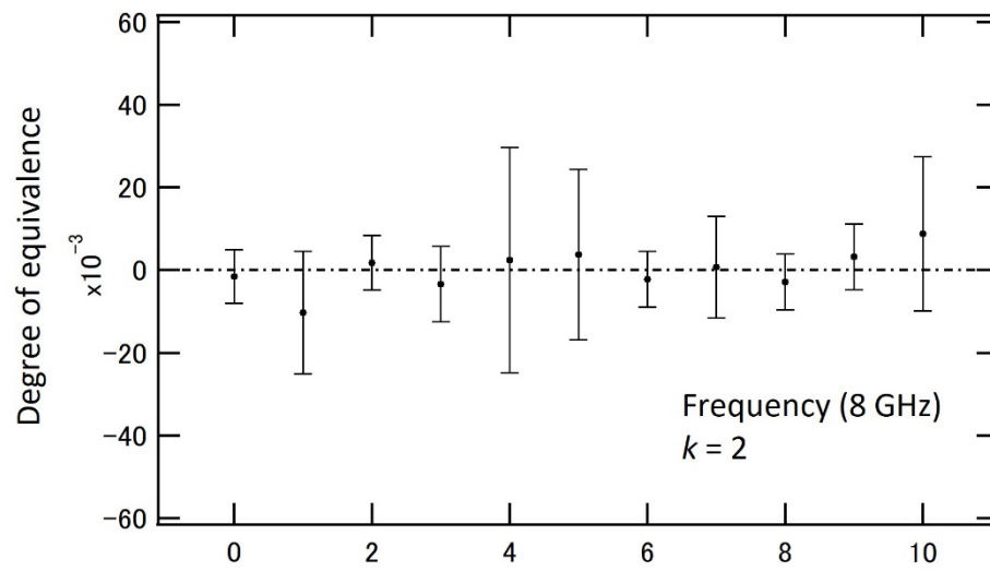
Fig. 9.5 DoE between m(L_i) and CCEM KCRV (8 GHz)
