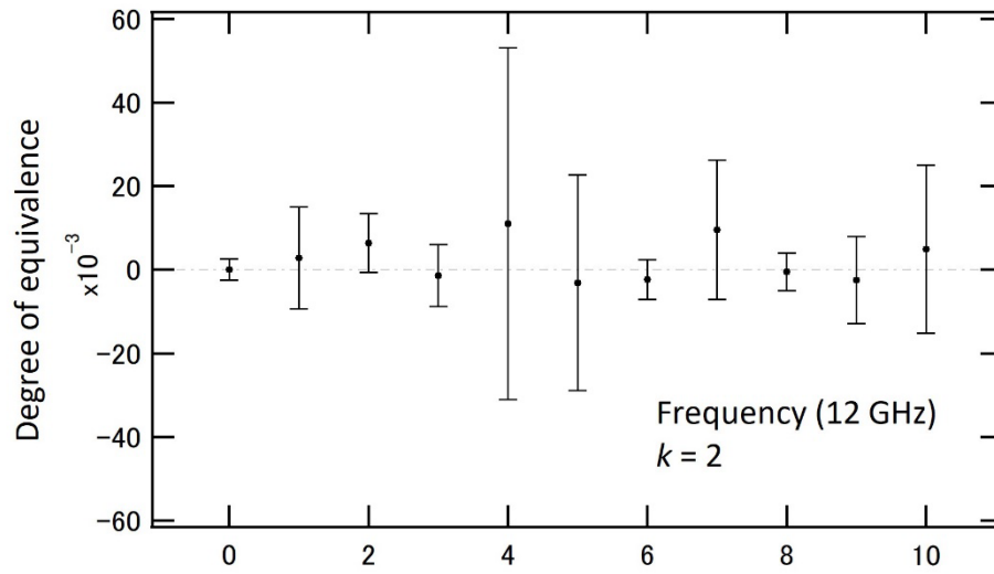
Fig. 8.12 DoE between m(L_i) and APMP RV (12 GHz, Sensor No. 2)
