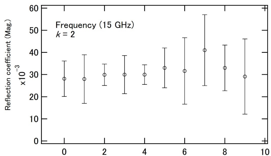
Fig. A.14 Reflection coefficient (15 GHz, Sensor No.2)
