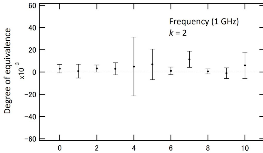
Fig. 9.3 DoE between m(L_i) and CCEM KCRV (1 GHz)
