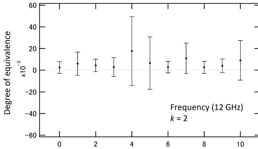
Fig. 9.6 DoE between m(L_i) and CCEM KCRV (12 GHz)
