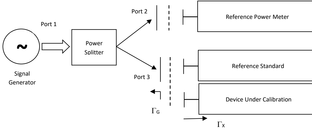
Fig.1: Coaxial Splitter based Power Measurement Setup
