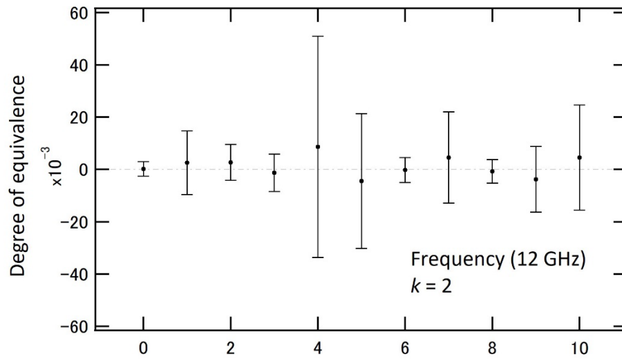
Fig. 8.11 DoE between m(L_i) and APMP RV (12 GHz, Sensor No. 1)
