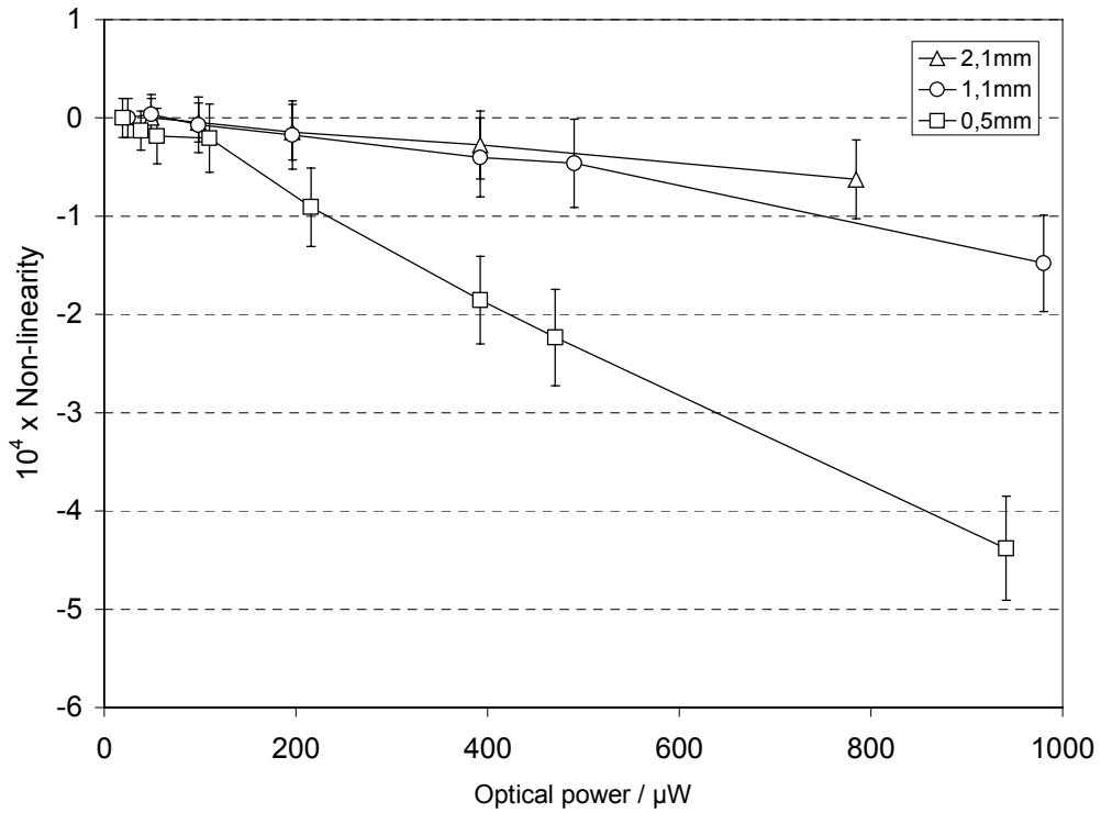
Figure 11 - Non-linearity of a transmission trap as a function of optical power for three different beam diameters ( 1/e^2 diameter) at \lambda = 633 \text{ nm} .
