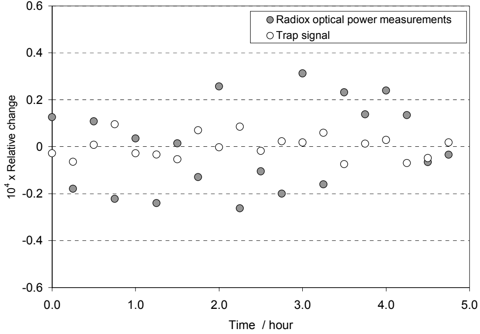
Figure 13 - Stability of the optical measurements during a calibration series at 514 nm (automated measurements performed during a single night).
