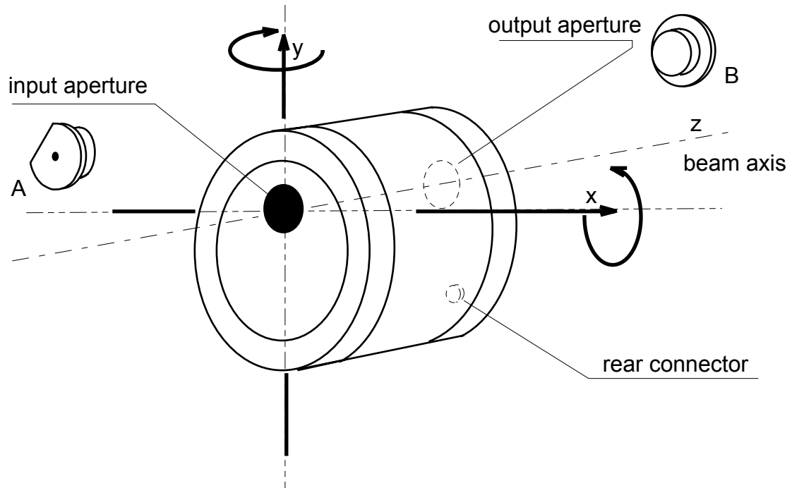
Figure 1. Alignment procedure for transmission traps.
