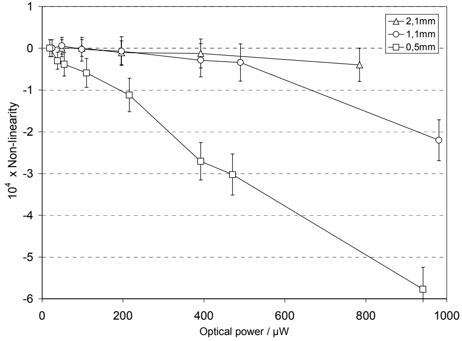
Figure 10 - Non-linearity of a reflection trap as a function of optical power for three different beam diameters ( 1/e^2 ) at \lambda = 633 \text{ nm} .
