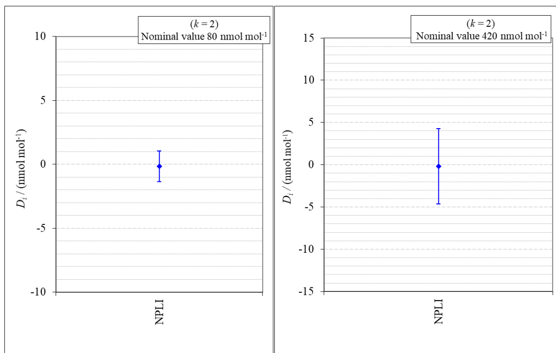
Figure 1: Degrees of equivalence of the NPLI at the two nominal ozone amount fractions 80 nmol mol -1 and 420 nmol mol -1
