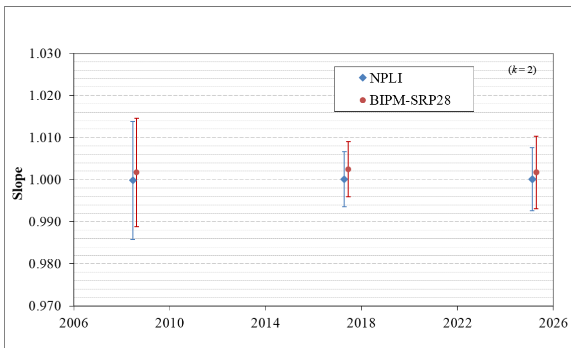
Figure 2: Results of previous comparisons between SRP27, SRP28 and NPLI-SRP43 realised at the BIPM. Uncertainties are calculated at k = 2 , with the uncertainty budget in use at the time of each comparison.
