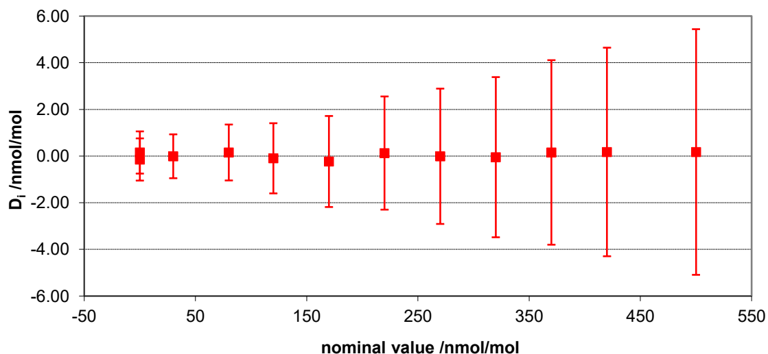
Degrees of equivalence at all measured values (k=2)
