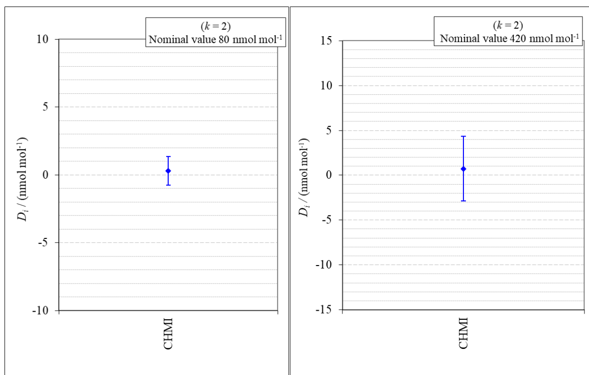
Figure 1: Degrees of equivalence of CHMI at the two nominal ozone amount fractions 80 \text{ nmol mol}^{-1} and 420 \text{ nmol mol}^{-1}
