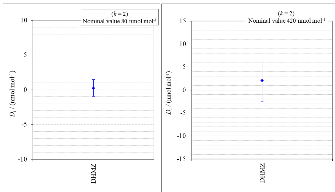
Figure 1: degrees of equivalence of the DHMZ at the two nominal ozone amount fractions 80 nmol mol -1 and 420 nmol mol -1
