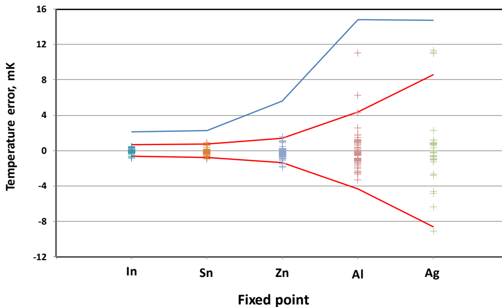
Figure 1: Summary of the measurements of the temperature errors in the 223 sealed fixed-point cells. The blue line shows the maximum error estimated according to Equation (A1.8), except for the silver cell, which is additionally assumed to have no gaseous oxygen present. The red lines show the k = 2 uncertainty envelope (see text).
