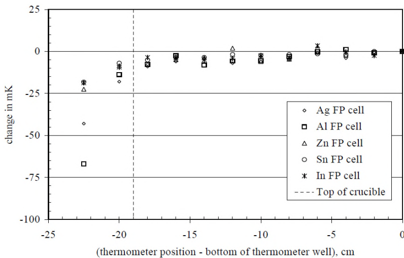
Figure 8. Vertical temperature profiles for several fixed-point cells, with furnace temperature 2.5 °C below the freezing point of the fixed-point cell. The thermometer position is relative to full insertion in the well [Strouse (2008)] 2 .
