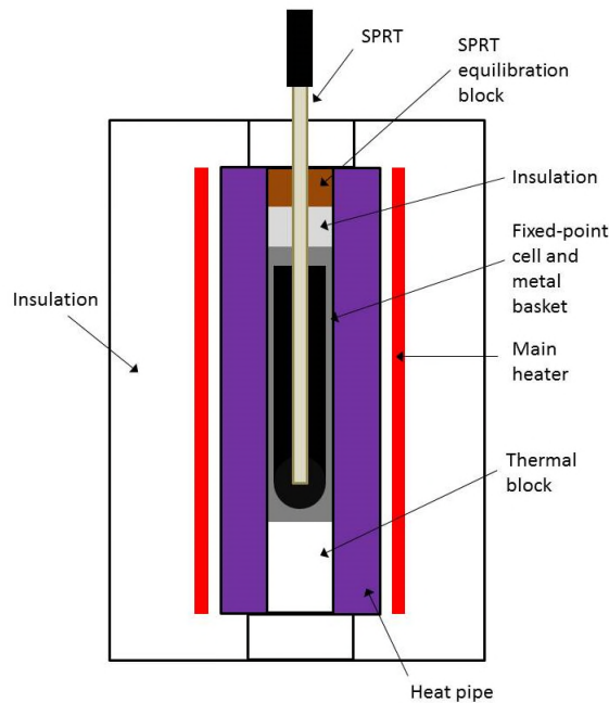
Figure 7. High temperature furnace for resistance thermometry metal freezing points. A heat pipe is preferred, but is a much more costly alternative to the Inconel block; with a heat pipe, the end heaters are omitted.
