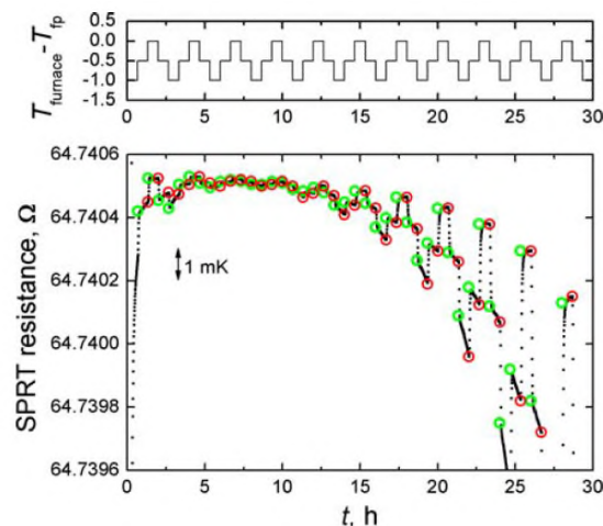
Figure 10. SPRT resistance as a function of time during Zn freeze, while the furnace temperature is oscillating by \pm 0.5 K, indicating a penetration ratio of \sim 0.01 . Illustration reproduced with the permission of Springer: International Journal of Thermophysics, “A New Method for the Quantification and Correction of Thermal Effects on the Realization of Fixed Points”, vol. 29, 2008, pp. 126-138, authors: M. Fahr and S. Rudtsch.
