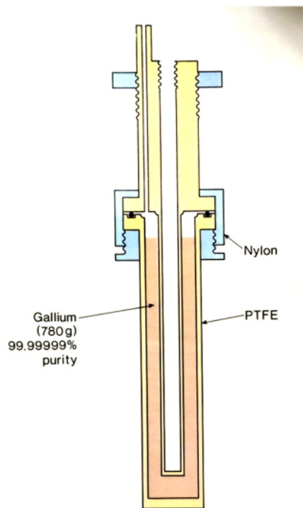
Figure 2. Gallium melting and triple-point cell.
