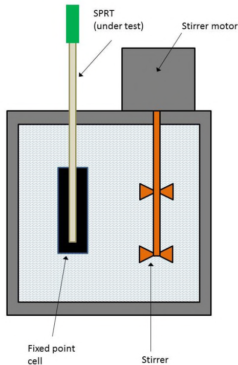
Figure 5. Typical stirred liquid bath.
