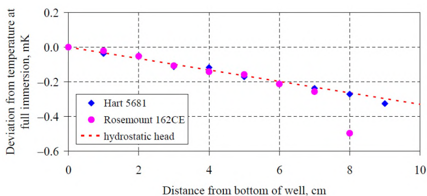
Figure 9. Immersion profile during realization of In freezing point [Strouse (2008)] 3 .
