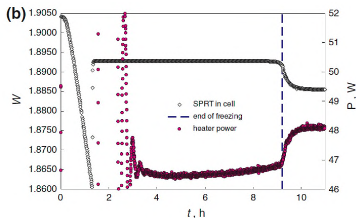
Figure 11. Determination of endpoint by measuring the heater power (lower trace) concurrently with the SPRT resistance (upper trace, resistance ratio W=R(t)/R(273.16\text{ K}) ); the abrupt increase in heater power at about 9 hours indicates the loss of heat flow from the ingot and therefore end of freezing. Illustration reproduced with the permission of Springer: International Journal of Thermophysics, “Thermal Analysis of the Heater-Induced Realization of the Tin Fixed Point”, vol. 28, 2007, pp. 1941-1956, authors: K. Yamazawa, J.V. Widiatmo, and M. Arai.
