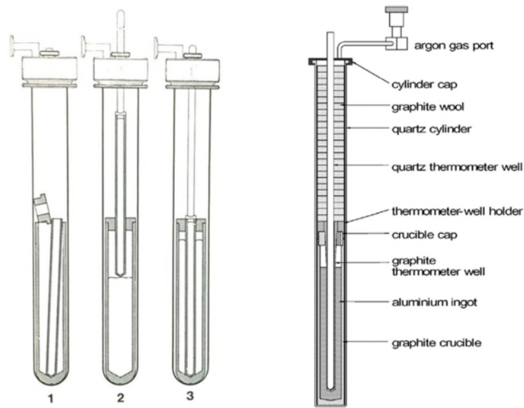
Figure 3. Open cell construction steps 1 to 3 (left [Nubbemeyer (1990)]) and finished assembly (right [Widiatmo et al. (2006)]). (Illustration to the right is reproduced by permission of IOP Publishing. All rights reserved. [Widiatmo et al. (2006)].)
