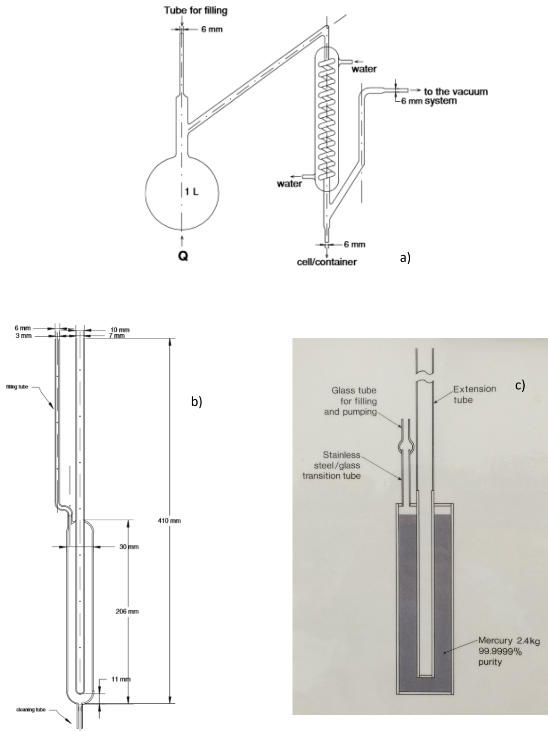
Figure 1. Distillation apparatus for mercury cells (a), and design (b) [del Campo et al. (2008)]. c) Stainless-steel mercury cell. Illustration reproduced with the permission of Springer: International Journal of Thermophysics, “Assembly and Study of Different Mercury Cells with Known Impurity Content and Isotopic Composition”, vol. 29, 2008, pp. 93-103, authors: D. del Campo, V. Chimenti, J. Reyes, J.A. Rodriguez Castillon, M. Moldovan and J.I. Garcia Alonso.
