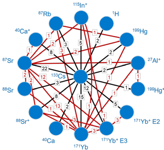
Figure 1: Representation of the 146 measurements linking 14 transitions on the circle and ^{133}\text{Cs} at the centre.
