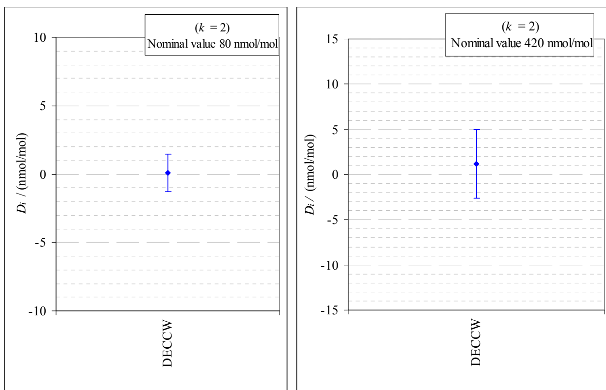
Figure 1: Graphs of equivalence of the DECCW at the two nominal ozone amount-of-substance fractions 80 nmol/mol and 420 nmol/mol
