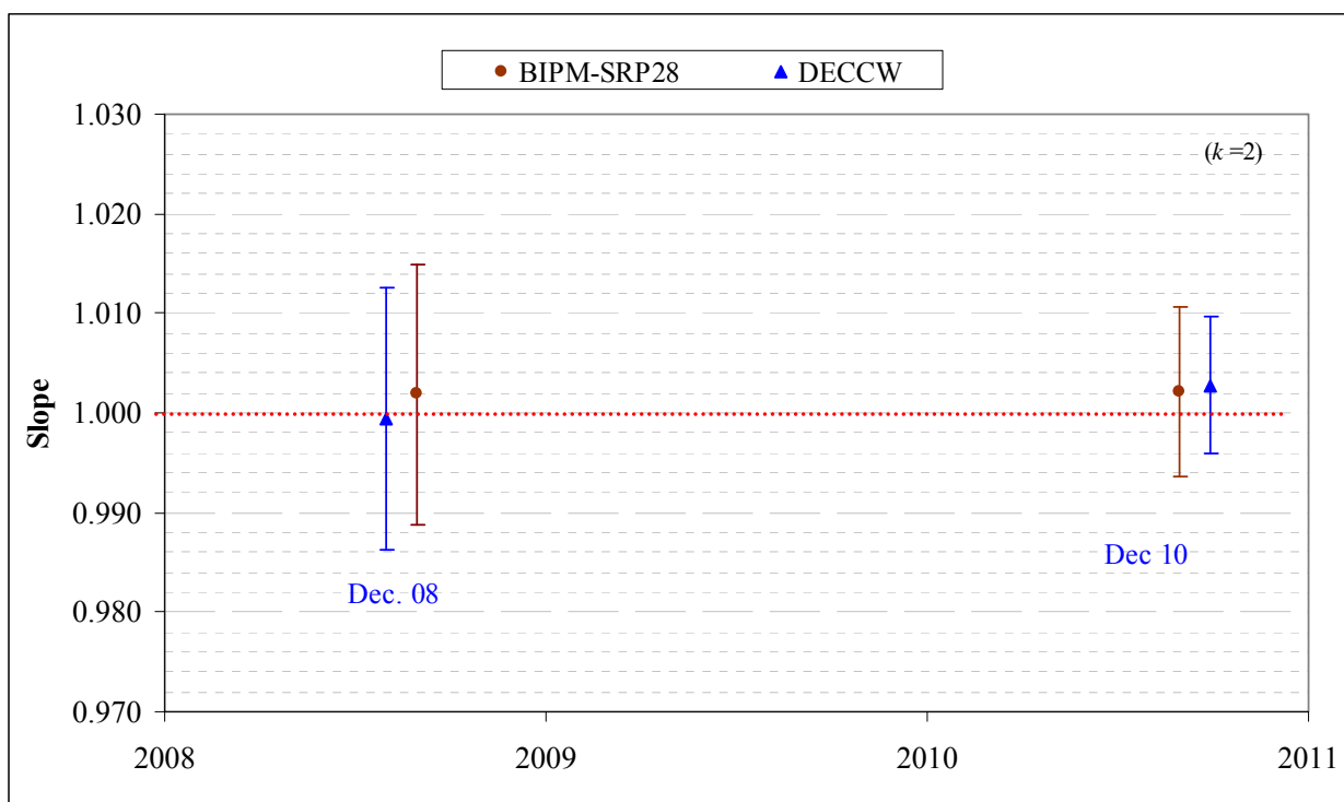
Figure 2 : Results of the comparisons between SRP27, SRP28 and DECCW SRP21 performed at the BIPM during the course of the key comparison BIPM.QM-K1. Uncertainties are calculated at k=2 , with the uncertainty budget in use at the time of each comparison.
