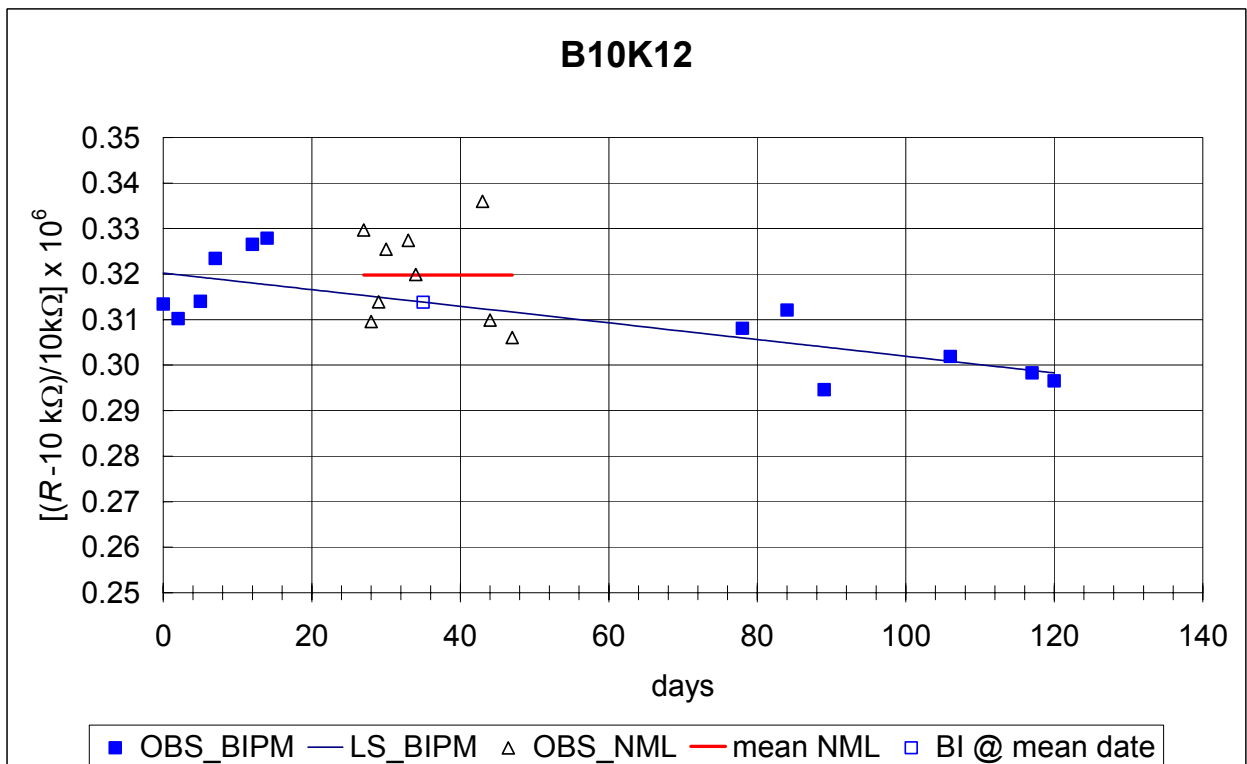
Figure 2. Relative deviation from the nominal 10 kΩ value of the resistance of B10K12 vs time: a linear least-squares fit (LS) to the BIPM measurements and the mean of the NML measurements.
