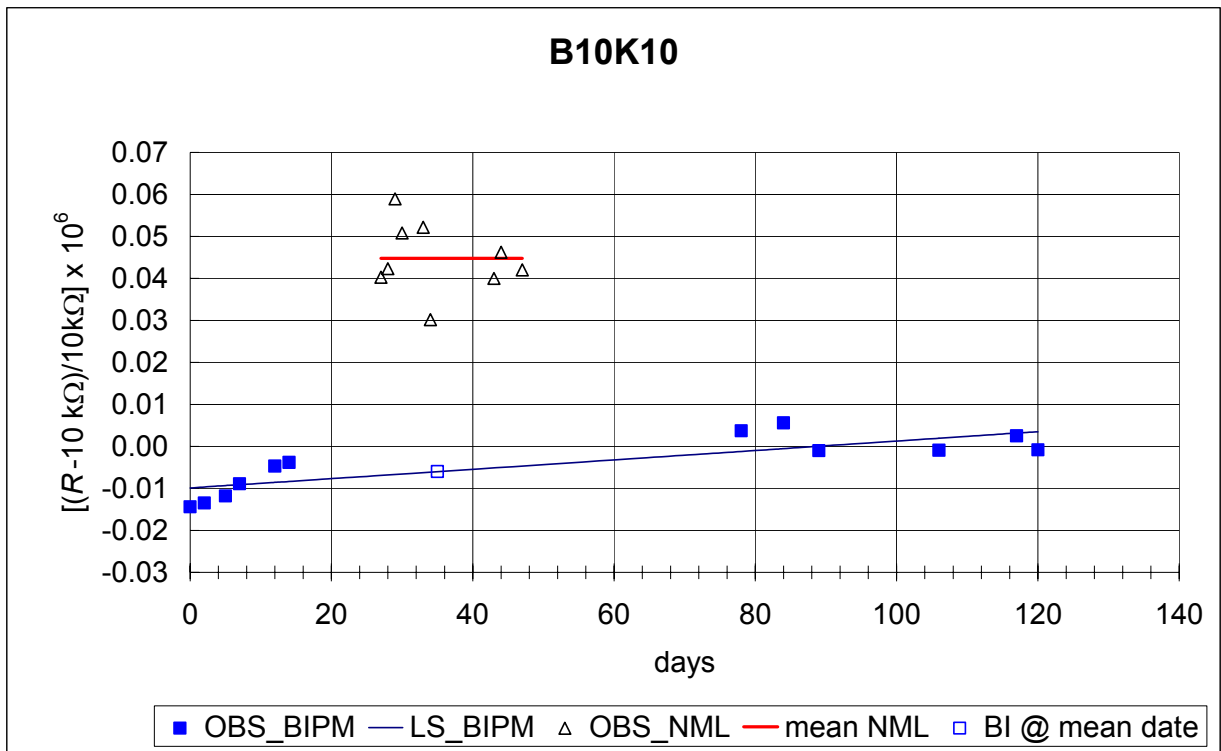
Figure 1. Relative deviation from the nominal 10 kΩ value of the resistance of B10K10 vs time: a linear least-squares fit (LS) to the BIPM measurements and the mean of the NML measurements.
