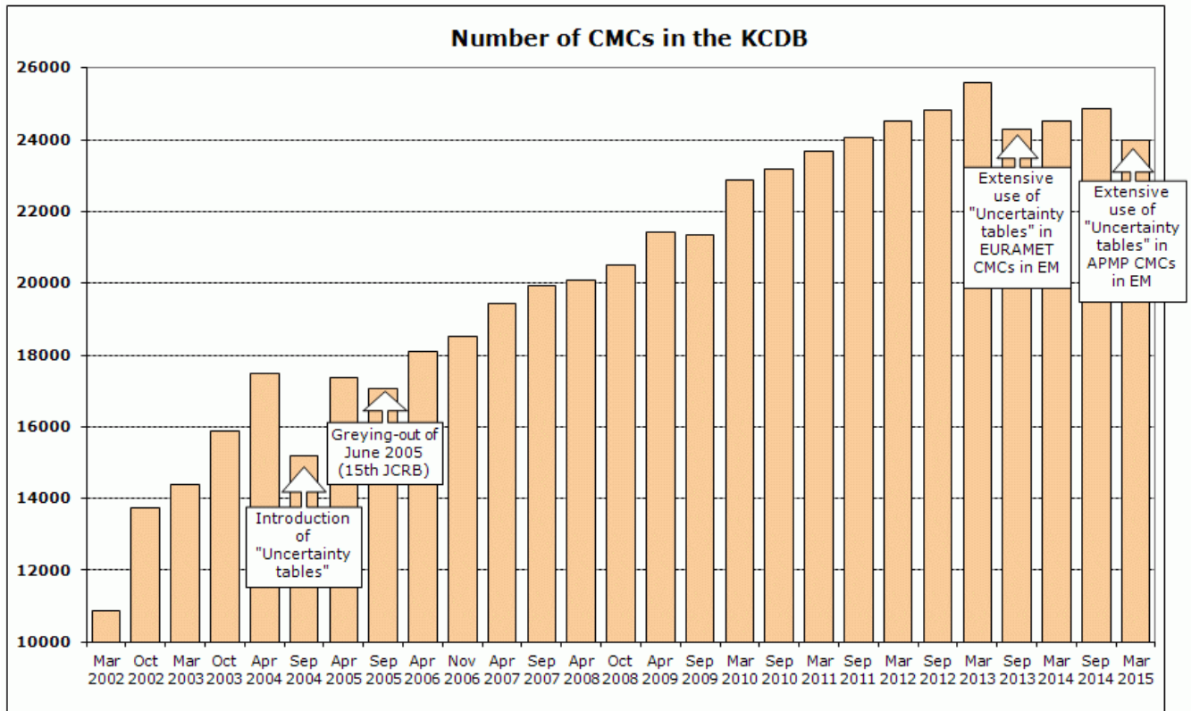
Fig 3 Evolution of the number of CMCs listed in the KCDB [4]
