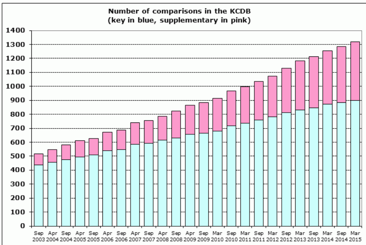
Fig 1 Total number of key comparisons and supplementary comparisons registered in the KCDB [4]
