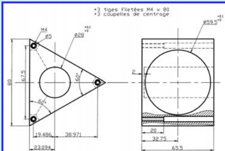
Source and photomultiplier holder
