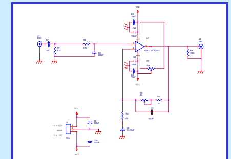
Diagram of a spectrometry preamplifier
