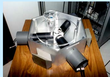
View of the counting set up
