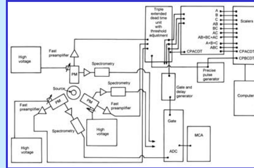
Schematic of experimental set up
