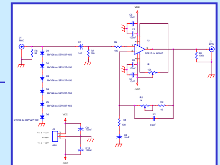
Diagram of an anode preamplifier
