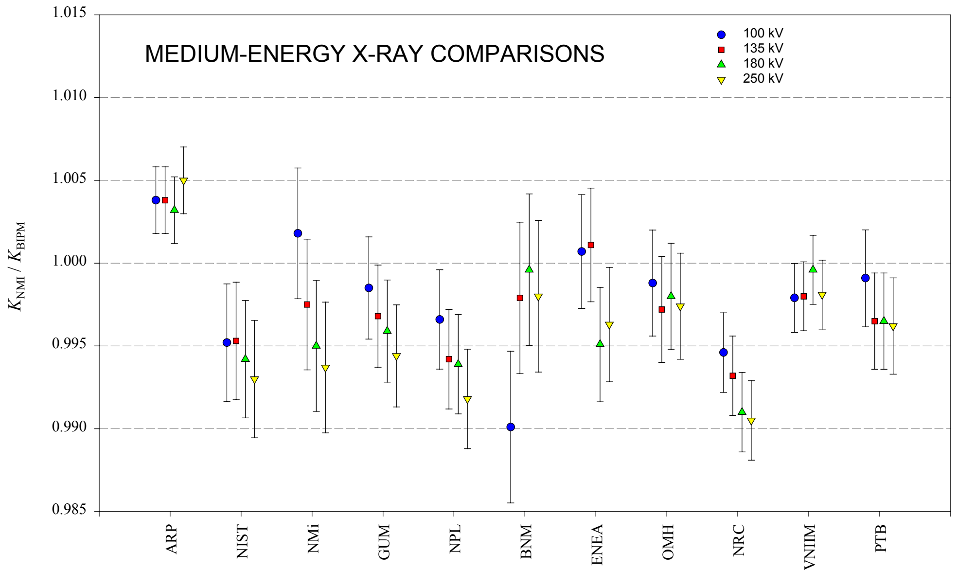
The results of BIPM medium-energy x-ray comparisons, expressed as the ratio K_{\text{NMI}} / K_{\text{BIPM}} of the air-kerma rate determined by the NMI standard to that determined by the BIPM standard. The uncertainty bars represent the standard uncertainty of each comparison result.
