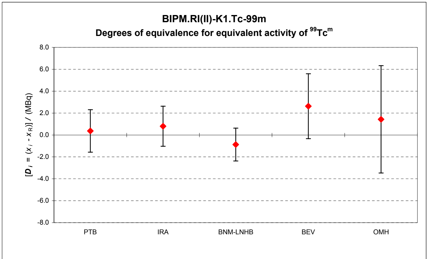
Figure 1. Graph of degrees of equivalence with the KCRV for ^{99}\text{Tc}^m (as it appears in Appendix B of the MRA)
