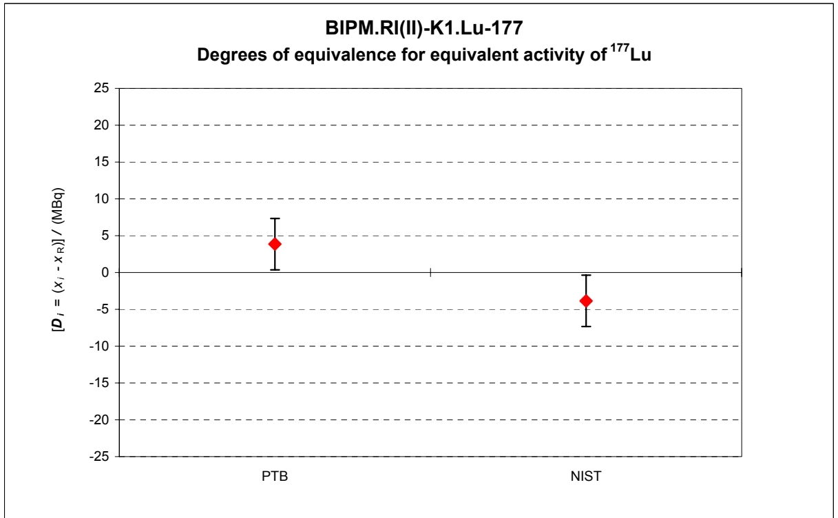
Figure 1. Graph of degrees of equivalence with the KCRV for ^{177}\text{Lu} (as it appears in Appendix B of the MRA)
