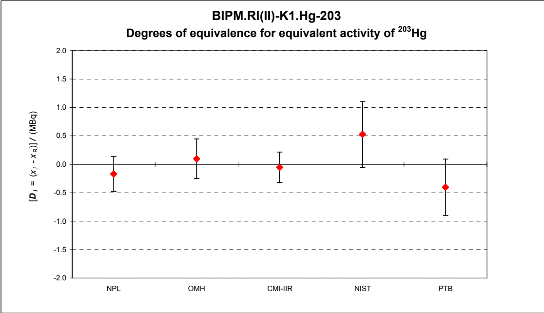
Figure 1. Graph of degrees of equivalence with the KCRV for ^{203}\text{Hg} (as it appears in Appendix B of the MRA)
