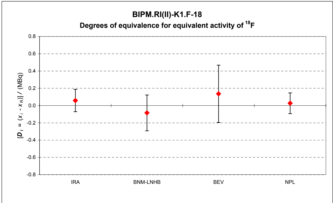
Figure 1. Graph of degrees of equivalence with the KCR (as it appears in Appendix B of the MRA)
