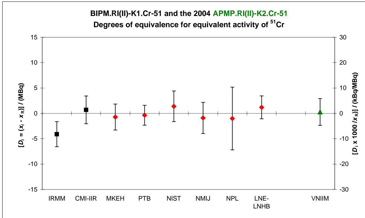
Figure 1. Graph of degrees of equivalence with the KCRV for ^{51}\text{Cr} (as it appears in Appendix B of the MRA)
