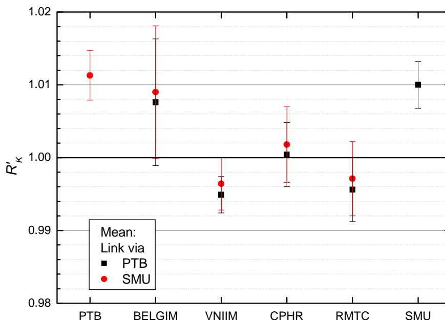
Figure 8. Comparison of the final results R'_K obtained from the link laboratories PTB and SMU based on the results of the mean values of the two transfer chambers.
