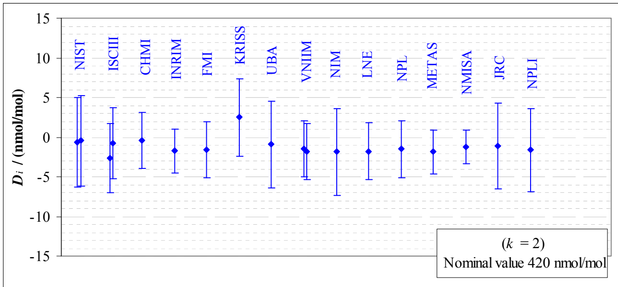
Figure 2: graphs of equivalence at the two nominal ozone mole fractions 80 nmol/mol and 420 nmol/mol, for all participants in BIPM.QM-K1 in the present cycle.
