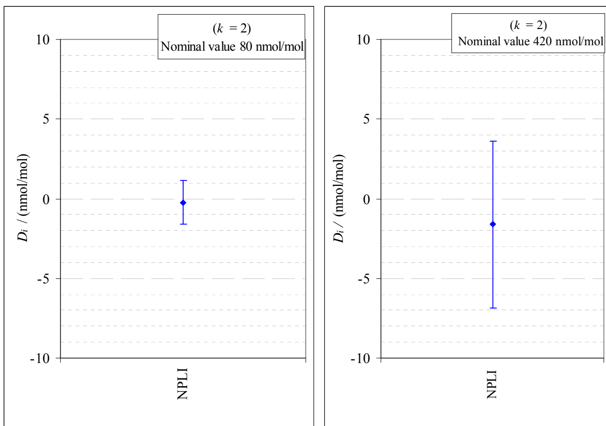
Figure 1: degrees of equivalence of the NPLI at the two nominal ozone mole fractions 80 nmol/mol and 420 nmol/mol
