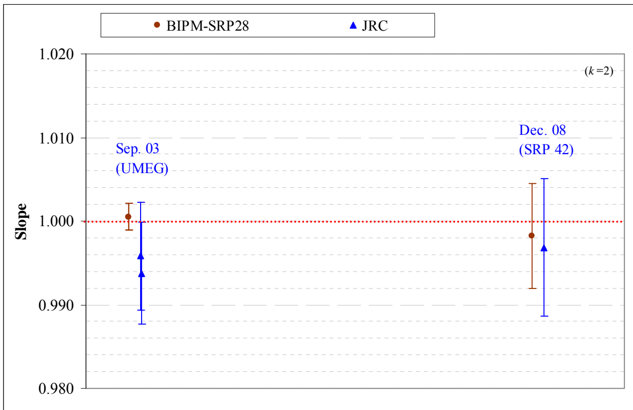
Figure 2: Results of the comparisons between SRP27, SRP28 and JRC-SRP42 realised at the BIPM during the pilot study CCQM-P28 and the key comparison BIPM.QM-K1. Uncertainties are calculated at k=2 , with the uncertainty budget in use at the time of each comparison. Note that the JRC national standard is not the same instrument in the two comparisons.
