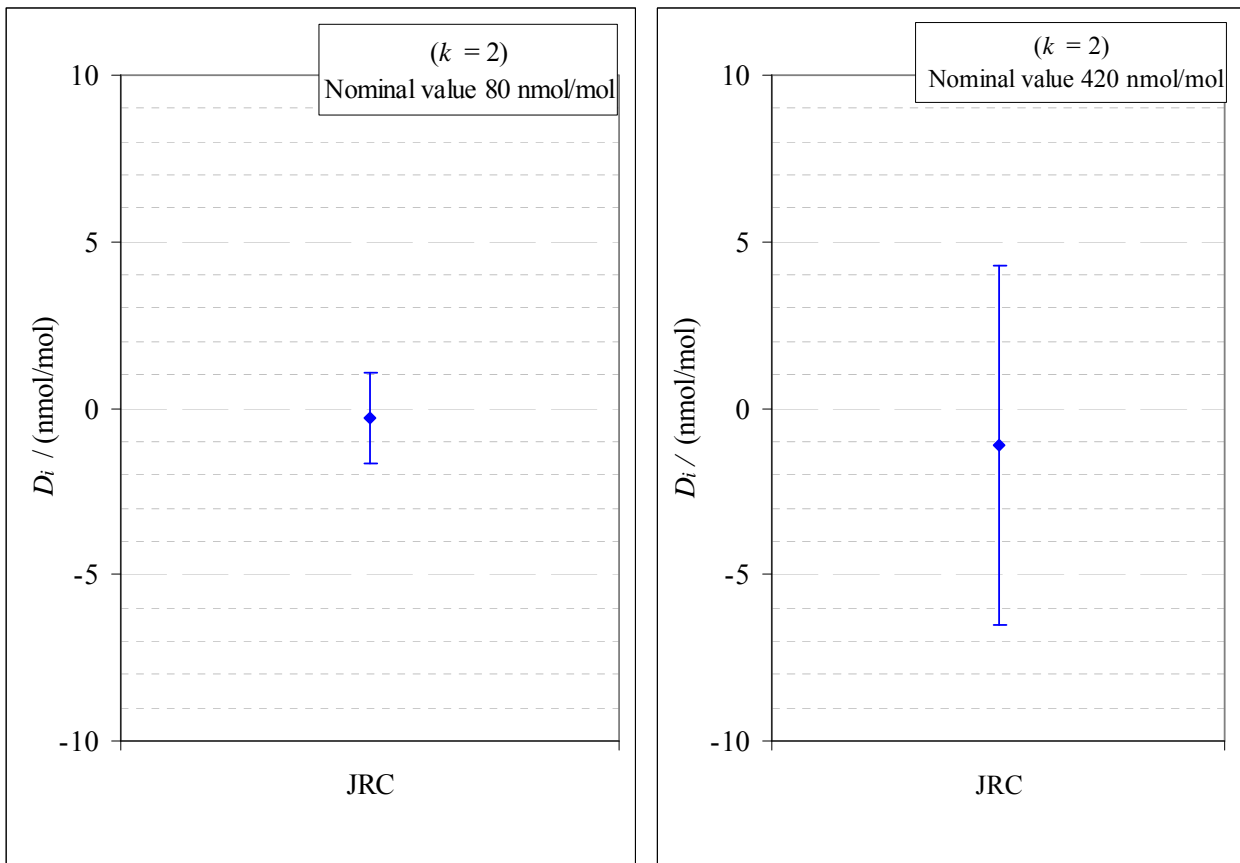
Figure 1: degrees of equivalence of the JRC at the two nominal ozone mole fractions 80 nmol/mol and 420 nmol/mol
