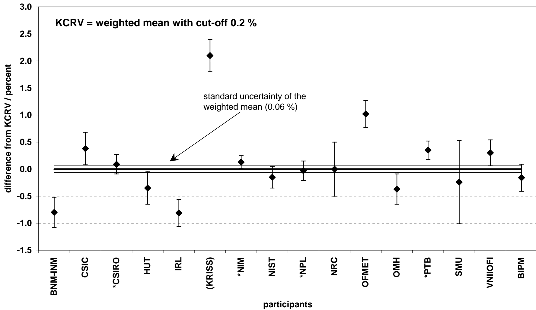
Figure 11: Results of the comparison averaged over all photometers per laboratory. The graph shows the relative difference from the weighted mean in percent for each laboratory. The uncertainties correspond to the standard uncertainties ( k=1 ) stated by the laboratories and do not include the uncertainty of the comparison itself.
