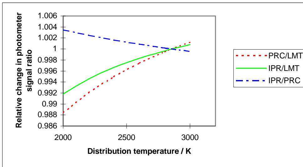
Figure 3b: Change in the measured ratio of photometer luminous responsivity as a function of distribution temperature.
