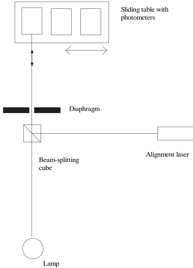
Figure 9: Photometer alignment.
