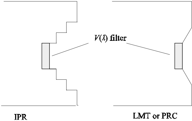
Figure 5: Shape of the front side of the photometers.
