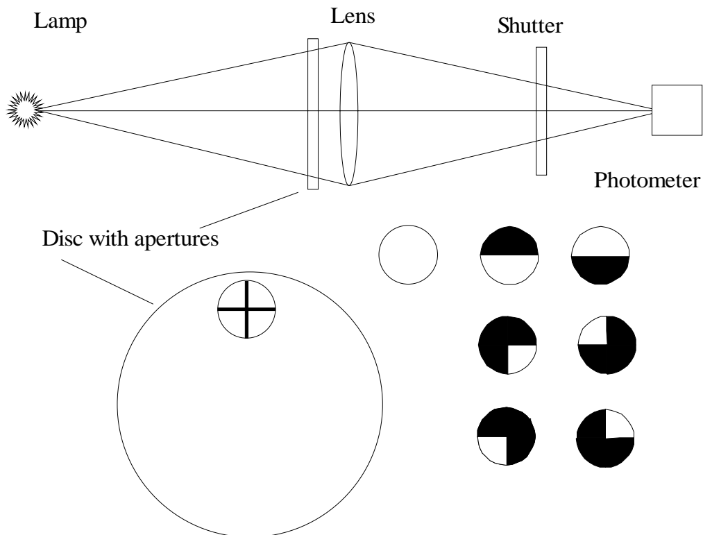
Figure 6: Set-up for the linearity measurement. Explanation in the text.
