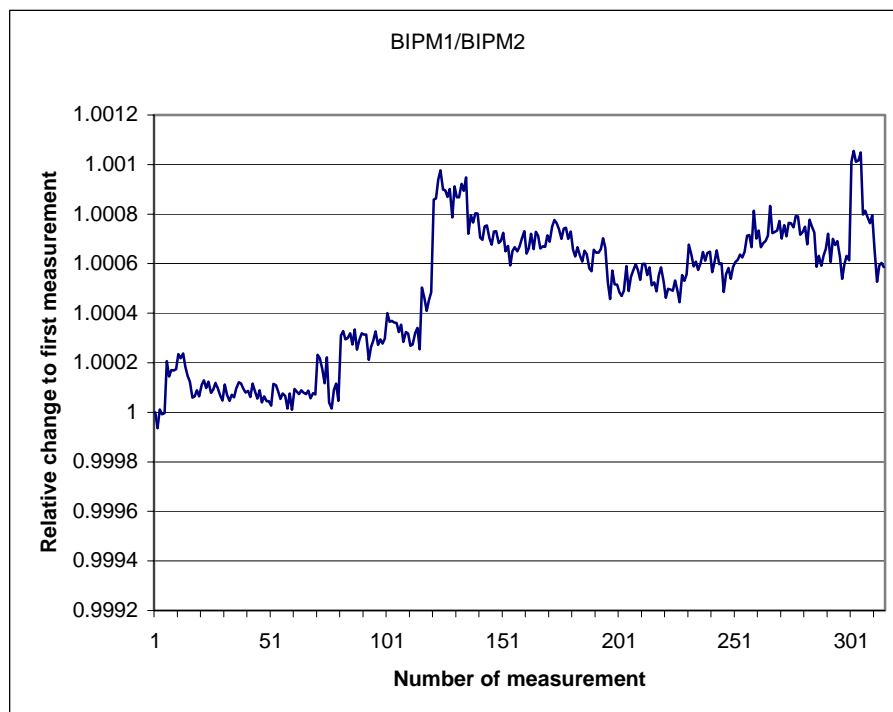
Figure 10a: Stability of the reference photometers, normalized ratio BIPM1 / BIPM2
