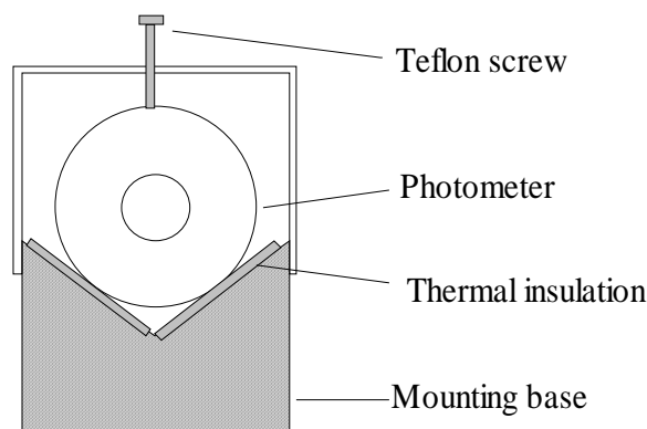
Figure 1: Thermal insulation of the photometer mount.
