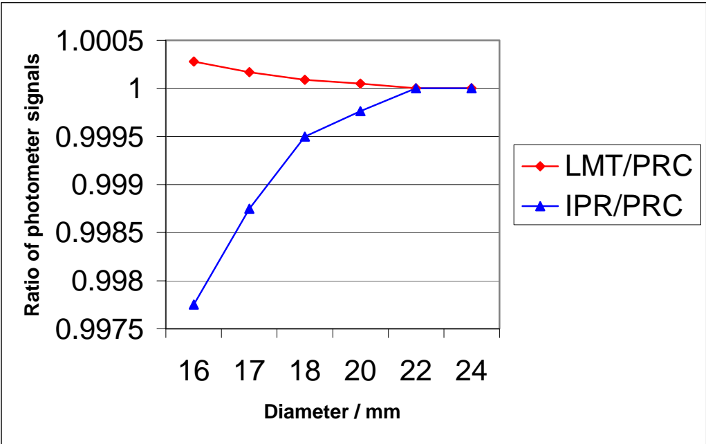
Figure 4: Influence of the aperture diameter on the photometer signal ratio.
