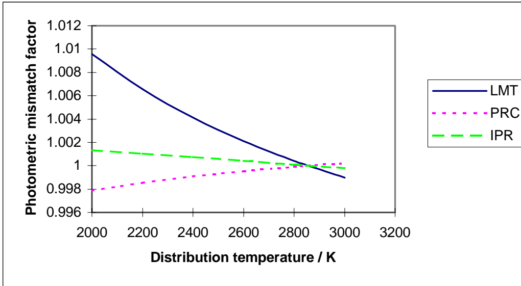
Figure 3a: Spectral mismatch for the BIPM photometers as a function of distribution temperature.
