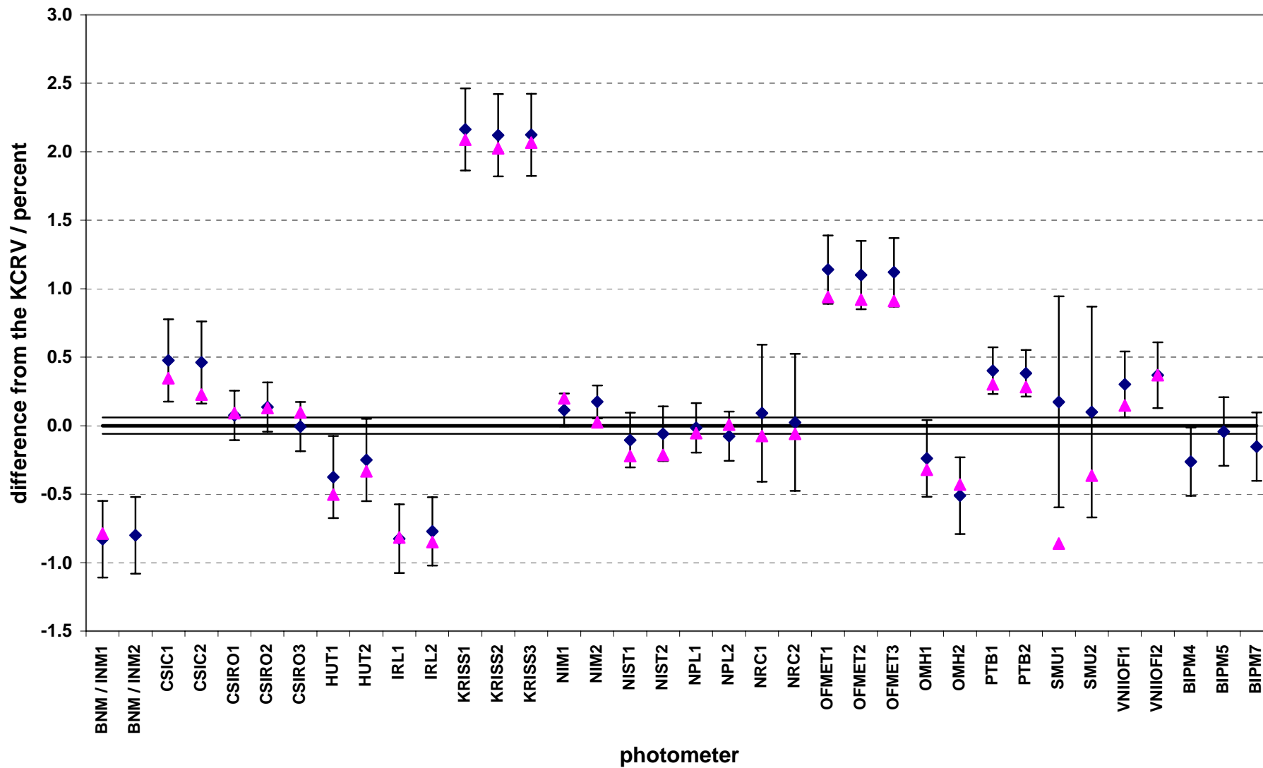
Figure 12: Results of the comparison for each individual photometer. The graph shows the relative difference from the same reference value as in Figure 11 in percent for each photometer before (diamonds) and after (triangles) the measurements at the BIPM. The uncertainties correspond to the standard uncertainties ( k=1 ) stated by the laboratories and do not include the uncertainty of the comparison itself.
