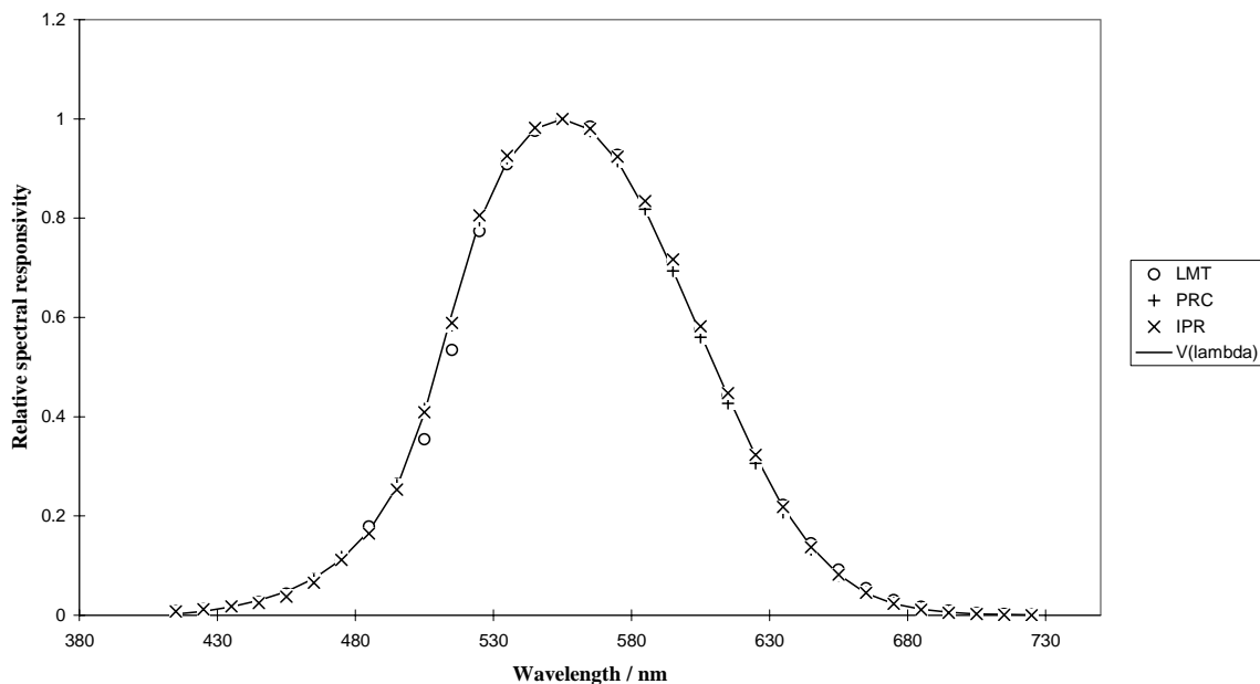
Figure 2: Relative spectral responsivities of the three BIPM photometers forming the reference group compared against V(\lambda) .
