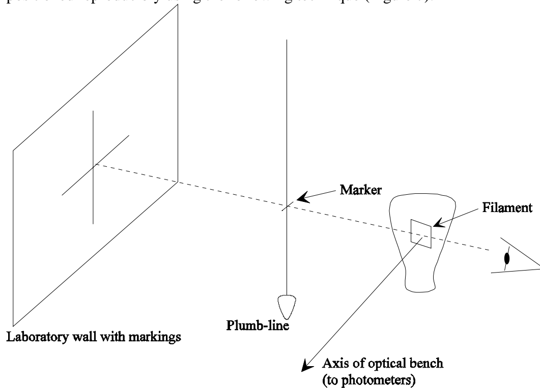
Figure 7: Method of lamp alignment.
