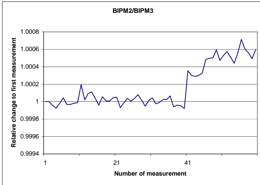
Figure 10b: Stability of the reference photometers, normalized ratio BIPM2 / BIPM3
