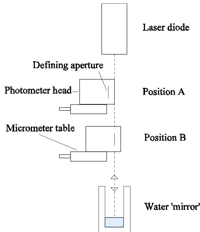
Figure 8: Alignment of the distance of the defining aperture.
