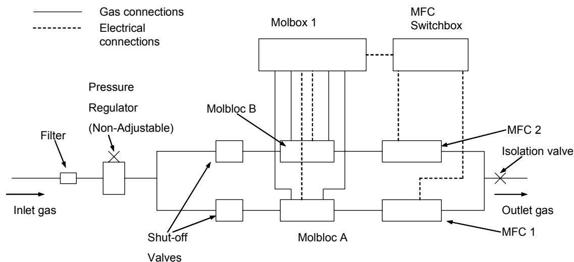
Figure 1 Schematic Diagram of the Transfer Standard
