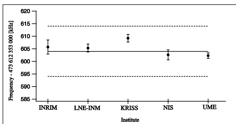
Figure 1. The final frequency values as given in column 3 in Table 4 for each laser. The solid line represents the present recommended value for the 633 nm laser standard and the dotted lines its uncertainty [1].
